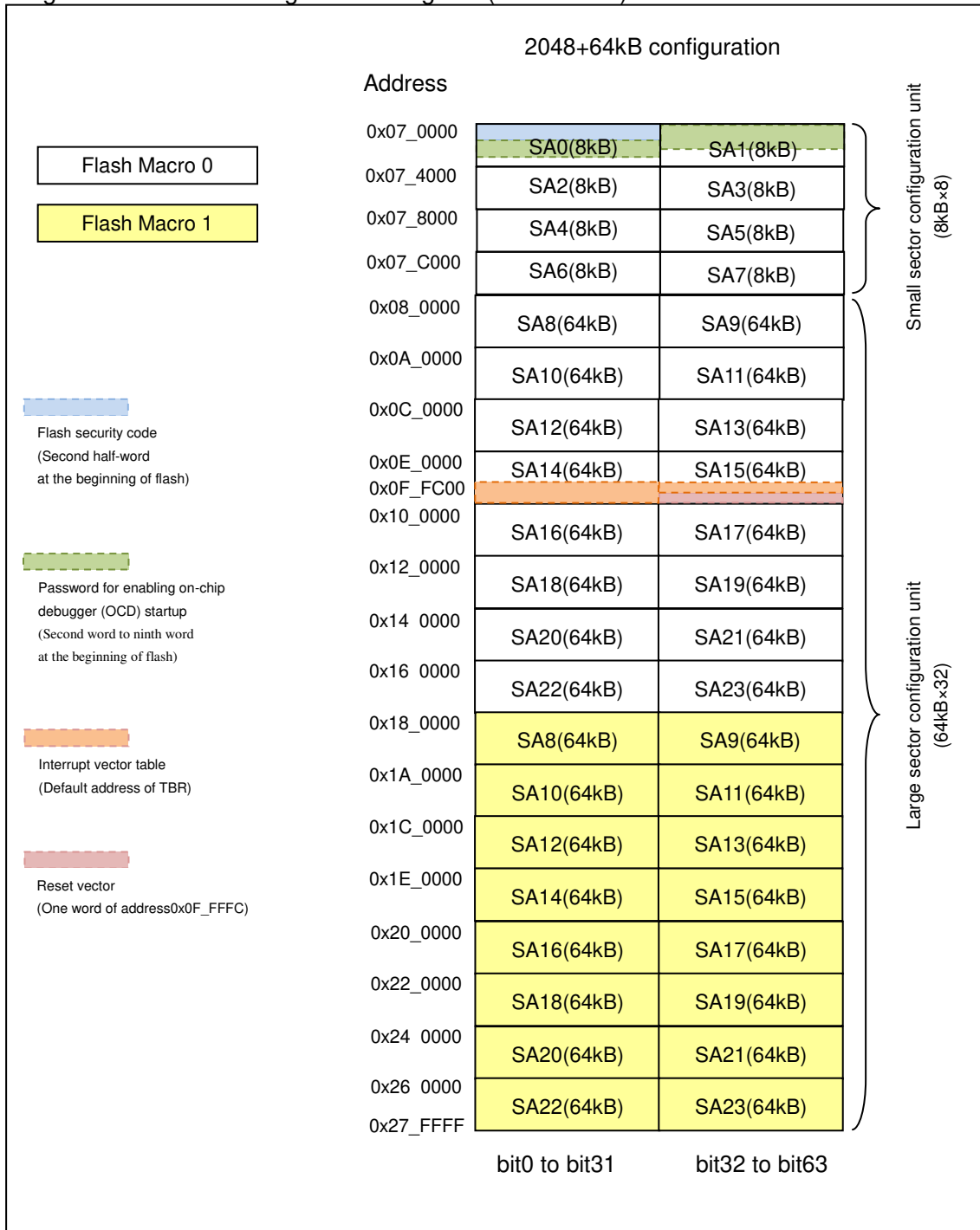
Figure 3-3 Sector Configuration Diagram (MB91F528)
