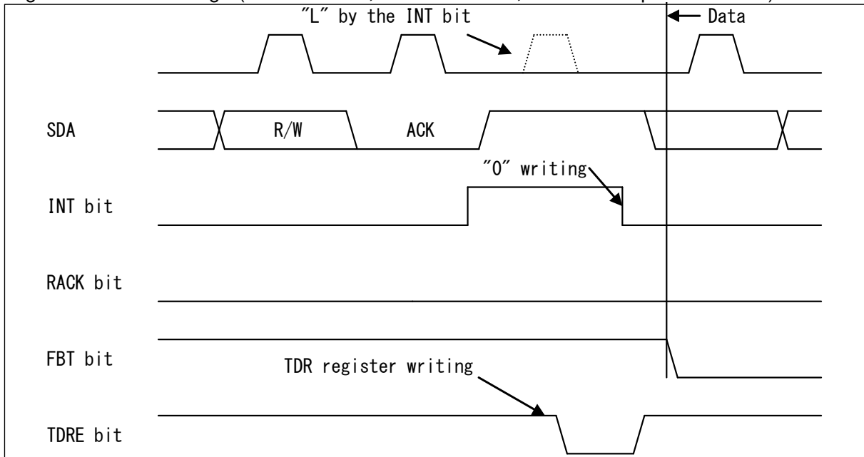
Figure 8-9 Acknowledge (FIFO Disable, IBSR:RSA="0", and the Response Is ACK)
