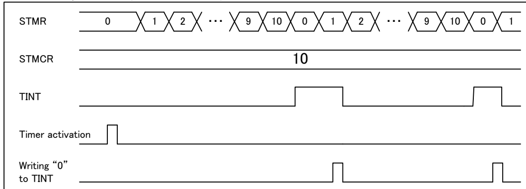
Figure 6-17 Timer Operation (STMCR="10")
