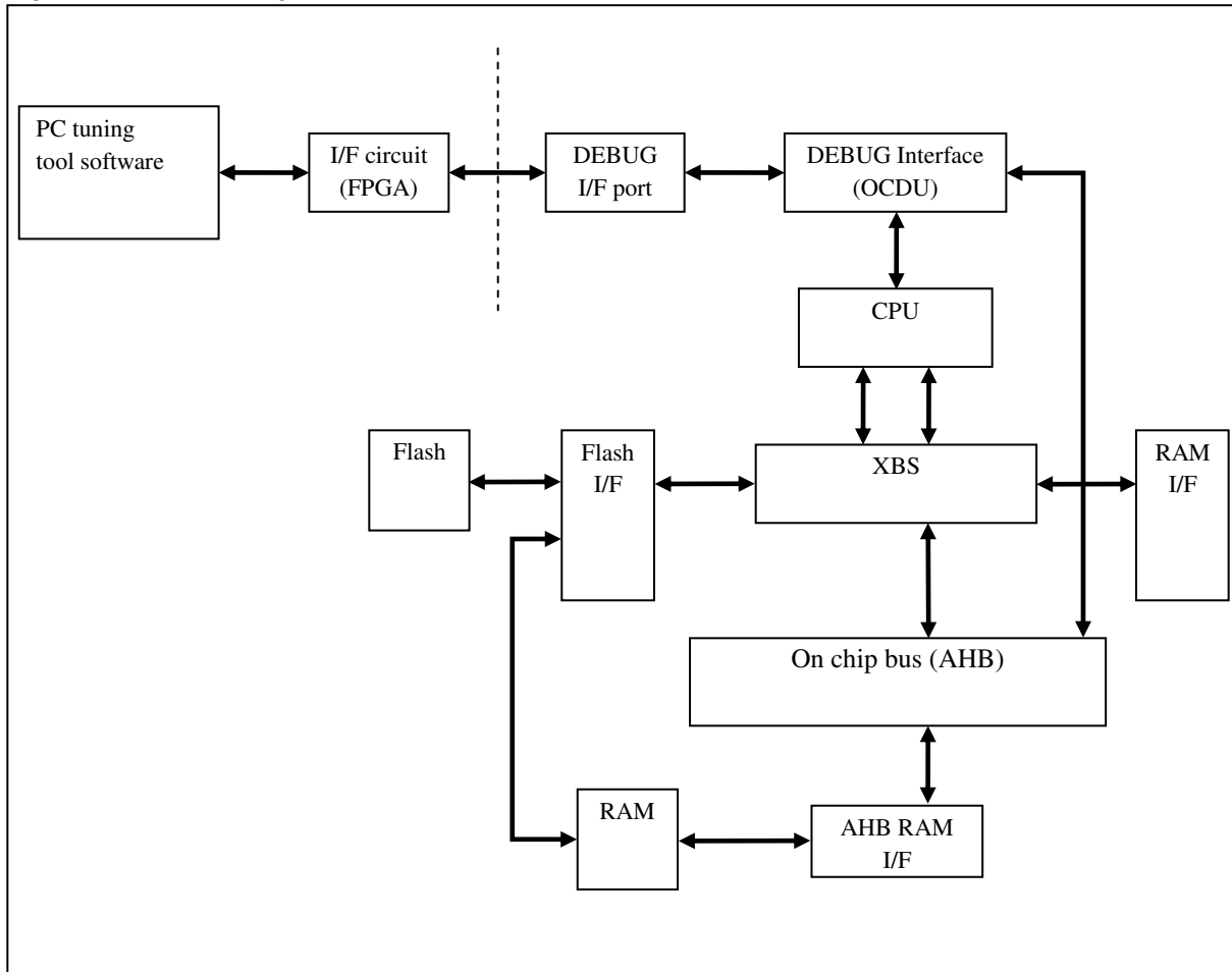
Figure 3-1 Block Diagram
