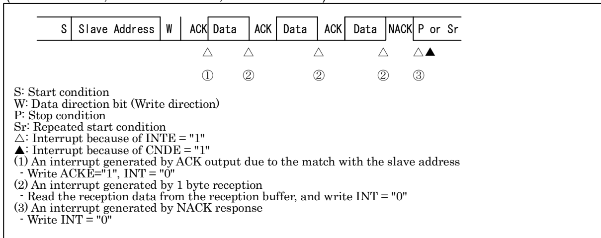
Figure 8-43 Slave Reception Interrupt (3)-when FIFO is Disabled (SSR:DMA="0", IBCR:WSEL="1", IBSR:RSA="0")
