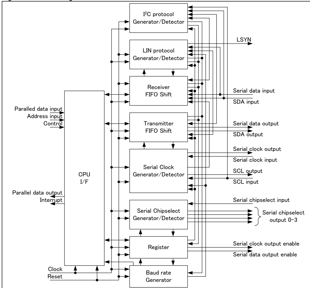
Figure 3-1 Block Diagram
