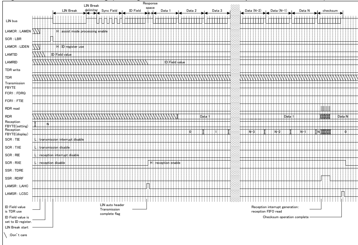
Figure 7-51 LIN Bus Timing (ID Register Use, DATA Field Reception, and FIFO Use)
