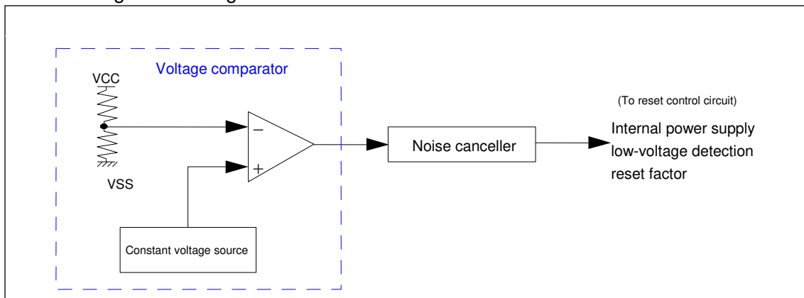
Figure 3-1 Configuration Diagram
