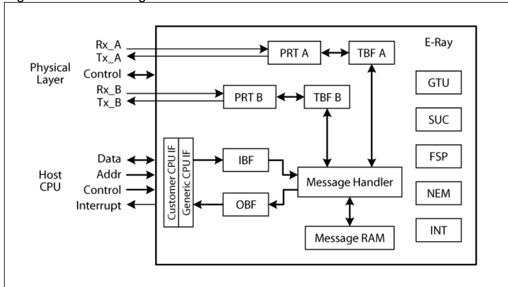
Figure 3-1 Block Diagram
