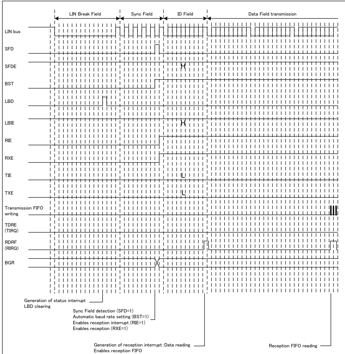
Figure 7-39 LIN Bus Timing (DATA Field Received: FIFO Used, AUTE=1)
