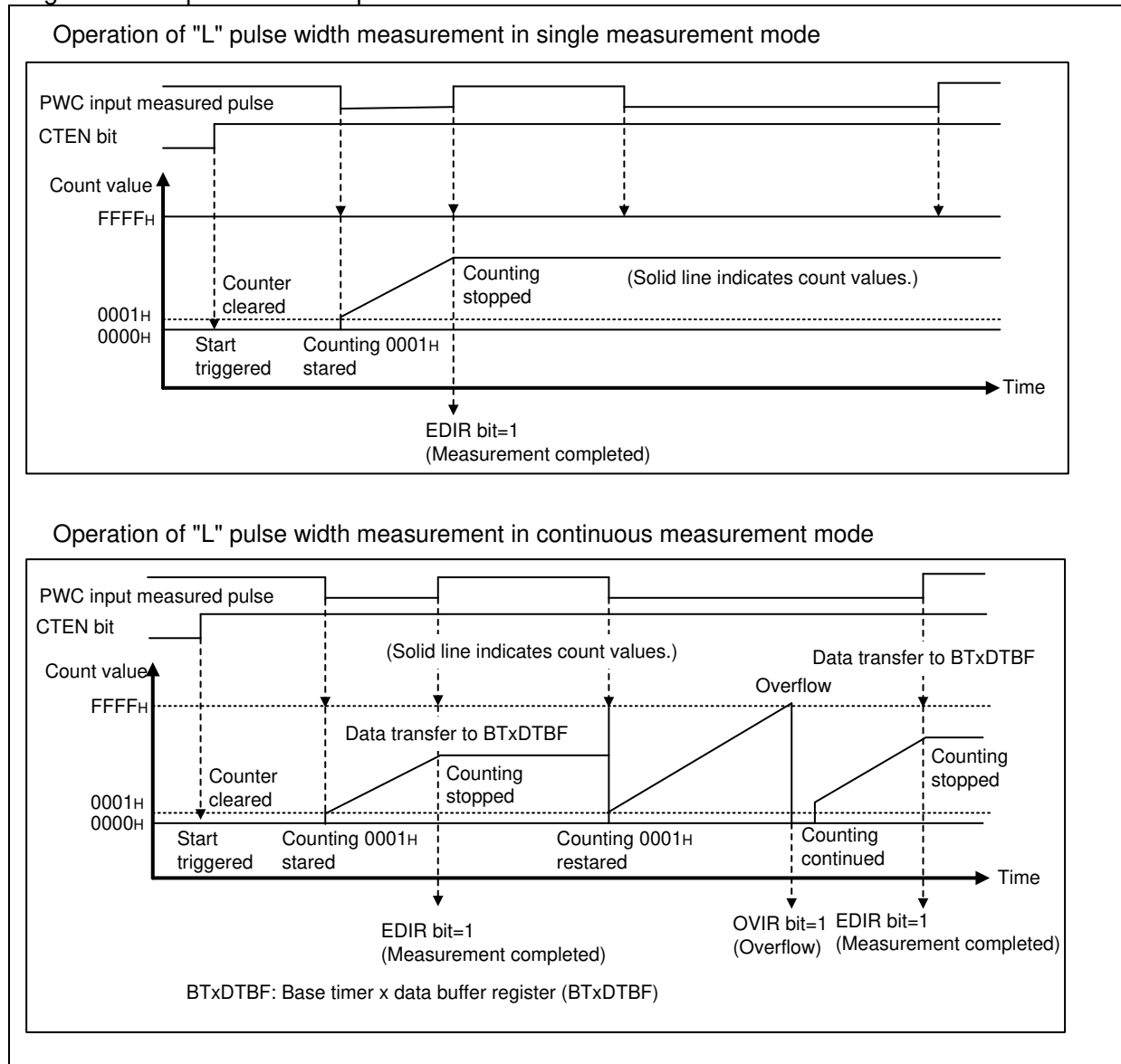
Figure 5-28 Operation Example
