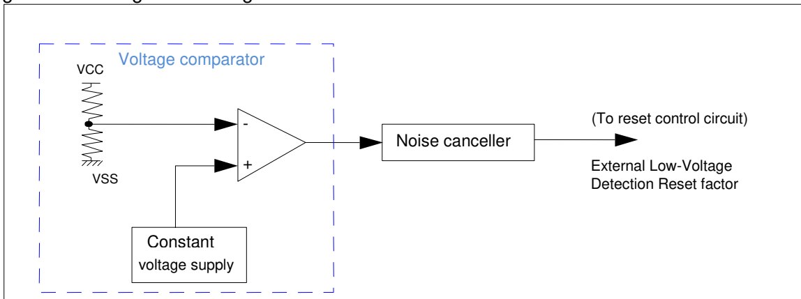
Figure 3-1 Configuration Diagram
