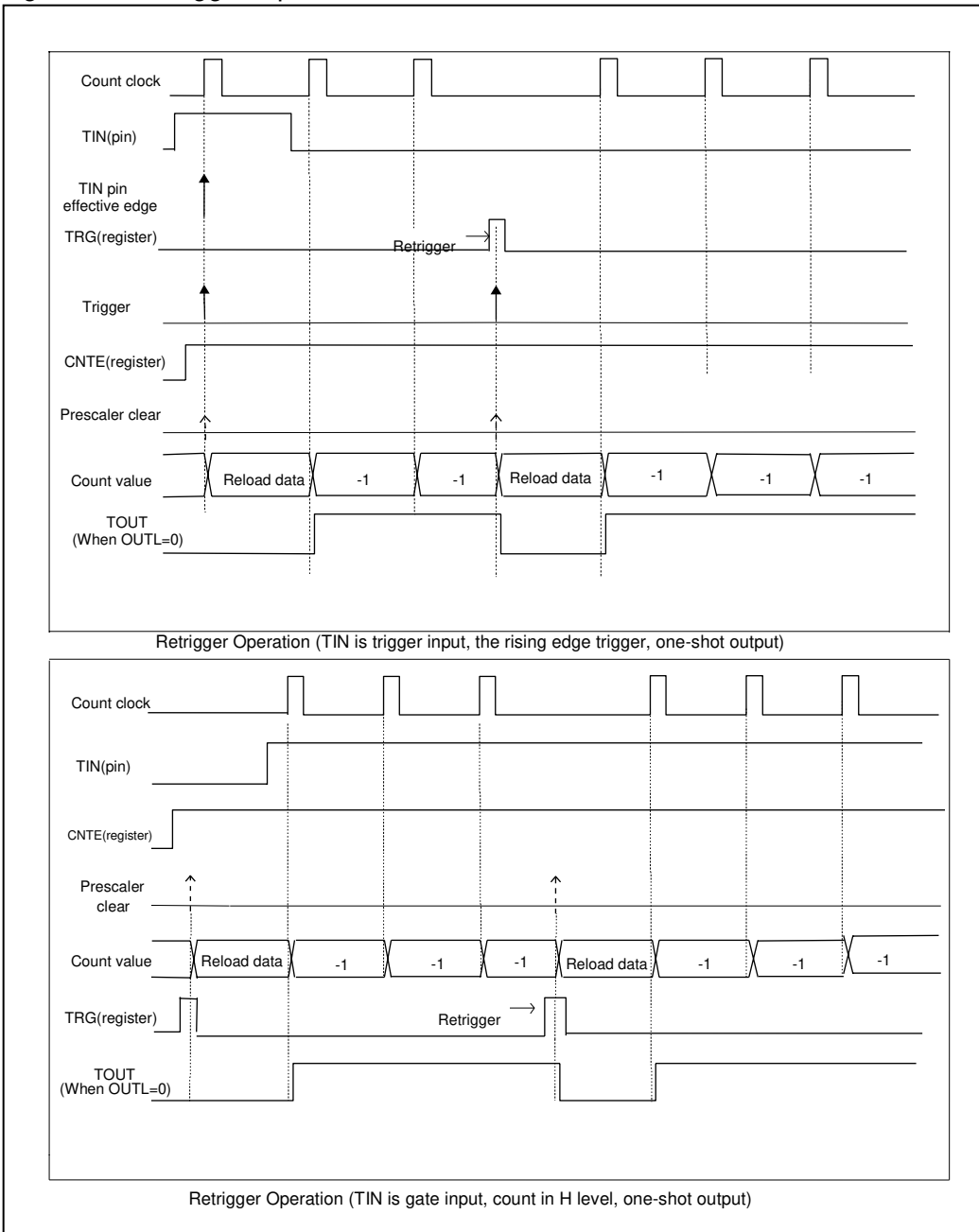
Figure 5-5 Retrigger Operation
