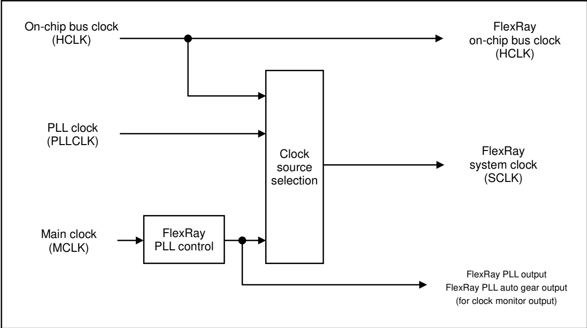
Figure 1-1 Block Diagram
