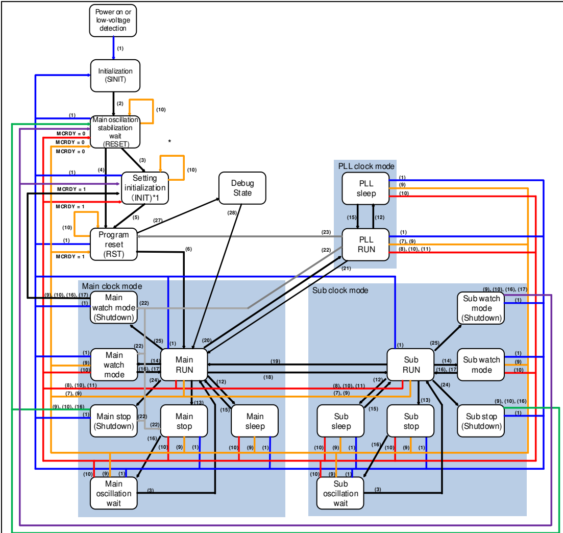
Figure 5-2 Device State
