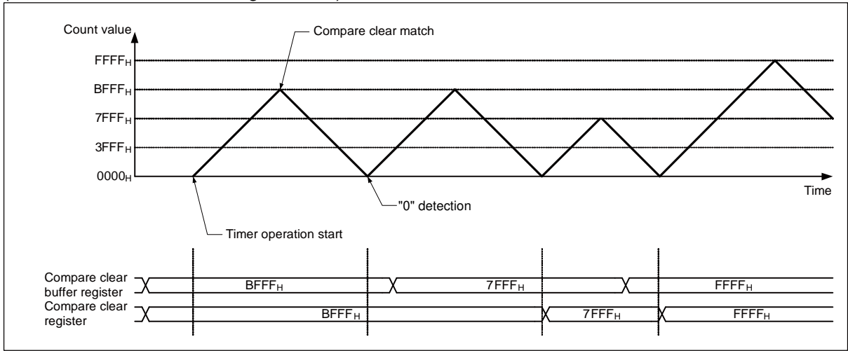
Figure 5-5 Operation in the Up/Down Count Mode when the Compare Clear Buffer is Enabled (BFE: bit23 of the TCCS register is 1)
