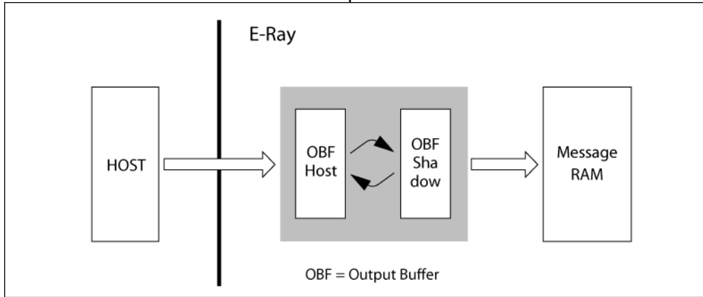
Figure 5-11 Double-buffer Structure of Output Buffer
