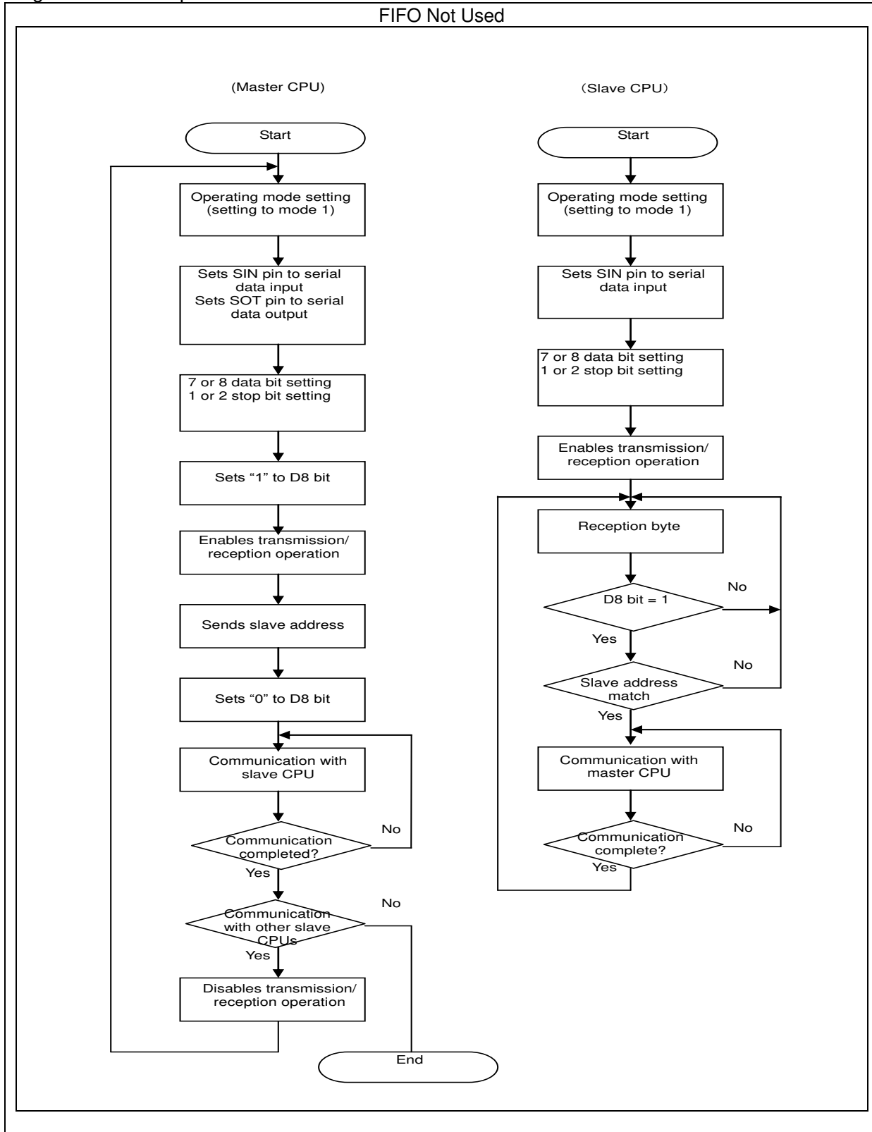
Figure 5-17 Example of Flowchart of Master-Slave Communications
