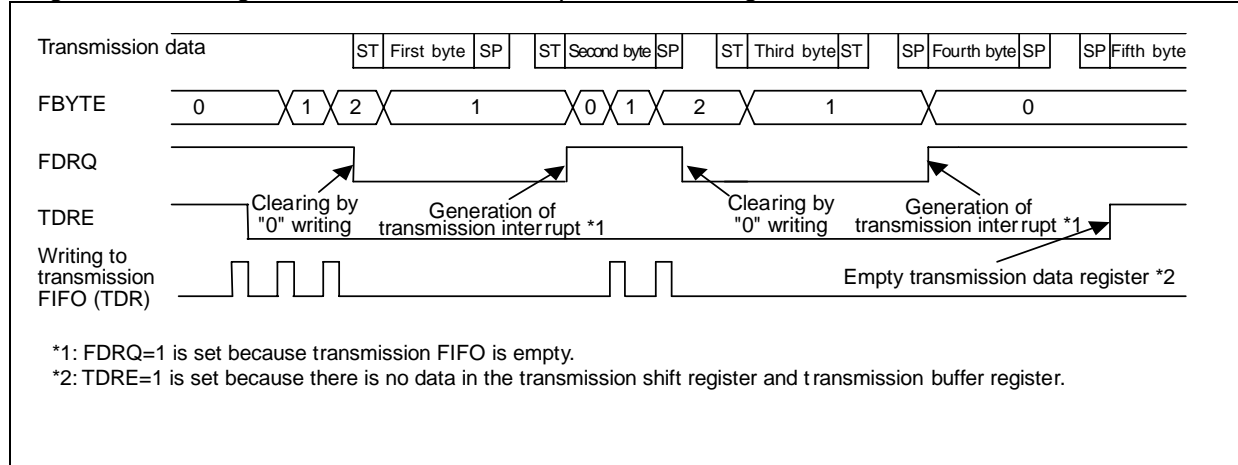
Figure 5-4 Timing of Transmission Interrupts when Using Transmission FIFO
