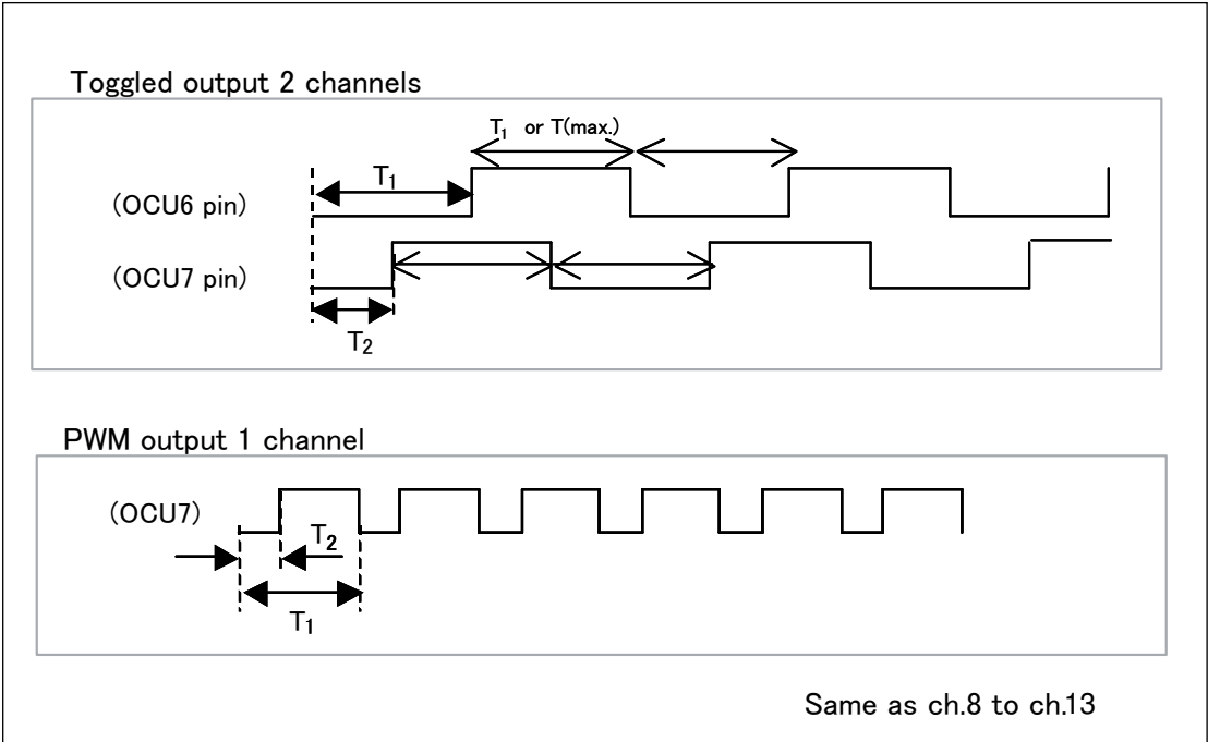
Figure 2-1 Output Waveform
