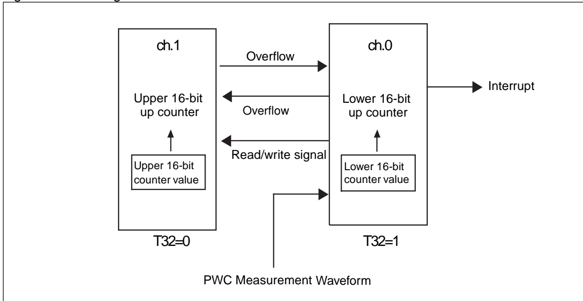
Figure 5-29 Configuration in 32-bit Timer Mode
