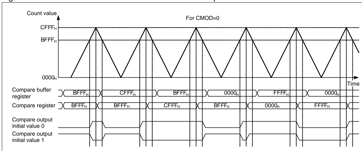
Figure 5-13 Case #1 Where the Free-run Timer Is in Up/Down Count Mode
