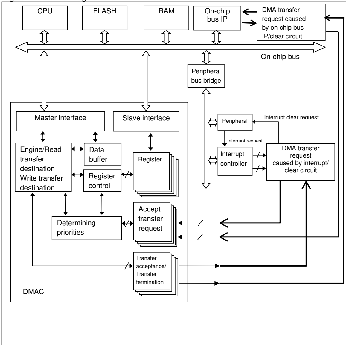
Figure 3-1 Block Diagram
