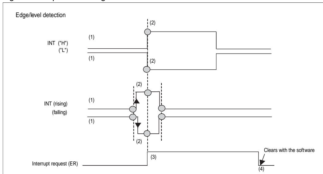
Figure 5-1 Operation Diagram
