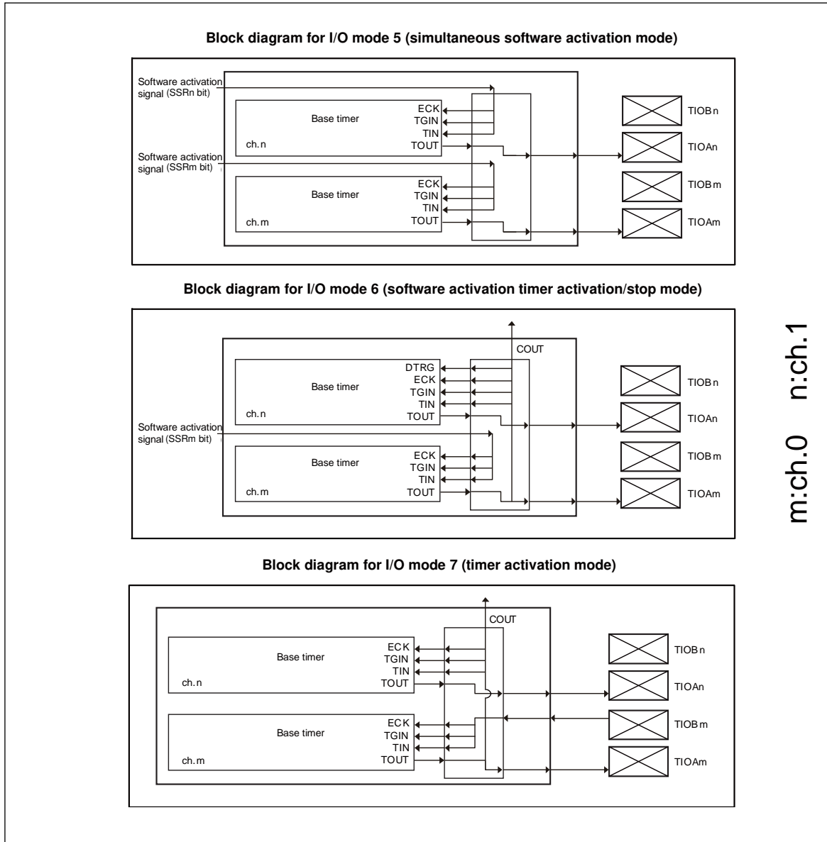
Figure 5-2 Wiring Diagram of Each I/O Mode (2)
