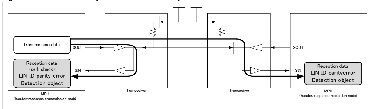
Figure 7-10 LIN ID Parity Error Detection Object
