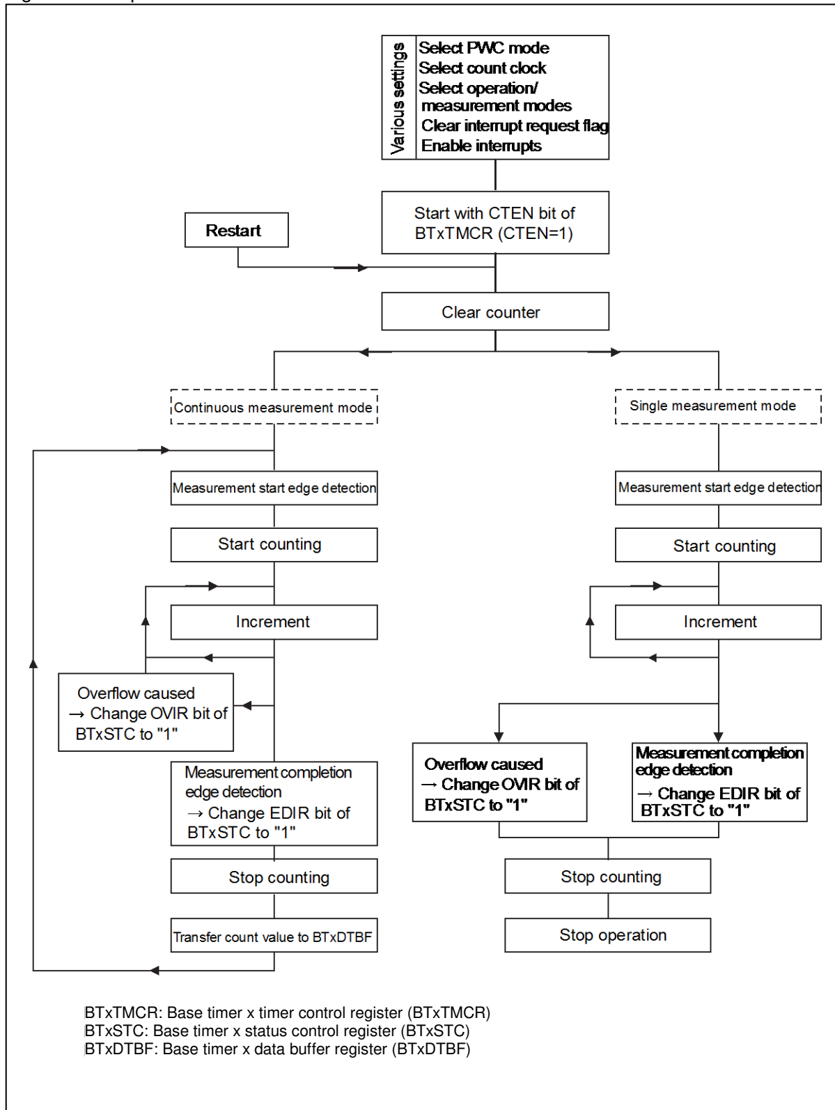
Figure 5-25 Operation Flow
