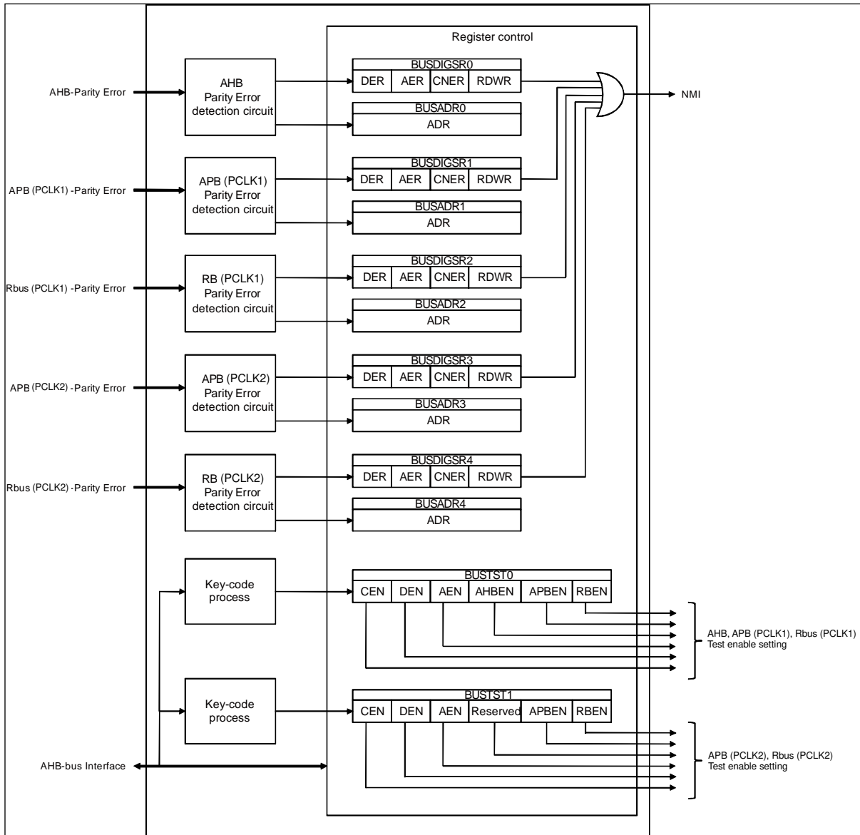
Figure 3-1 Configuration Diagram
