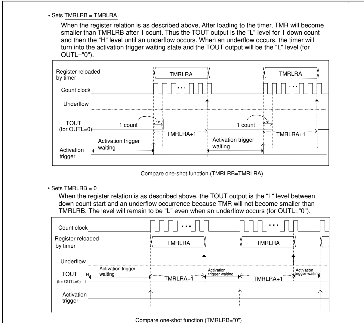
Figure 5-14 Compare One-shot Operation (2 / 2)
