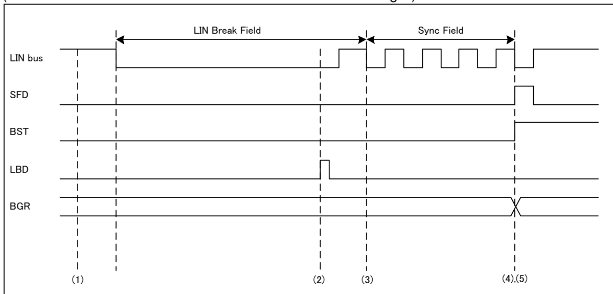
Figure 7-33 From LIN Break Field Reception to Sync Field Reception (in Case where STMR is SFUR or smaller and SFLR or larger)
