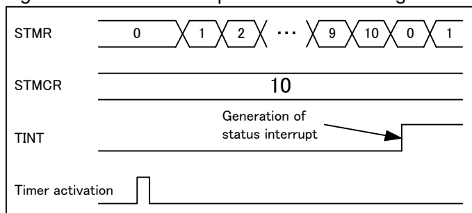
Figure 5-5 Timer Interrupt Generation Timing
