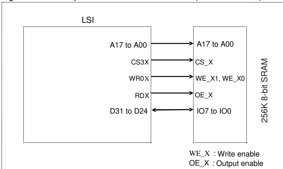
Figure 5-14 Example 2 of Connection to SRAM (8-bit SRAM x 1)
