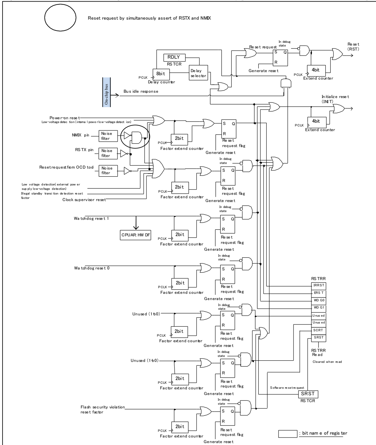
Figure 3-3 Configuration Diagram of Reset (Reset Control) [MB91F52xxxC/MB91F52xxxE]
