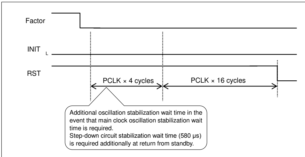
Figure 5-4 Reset (RST) Sequence
