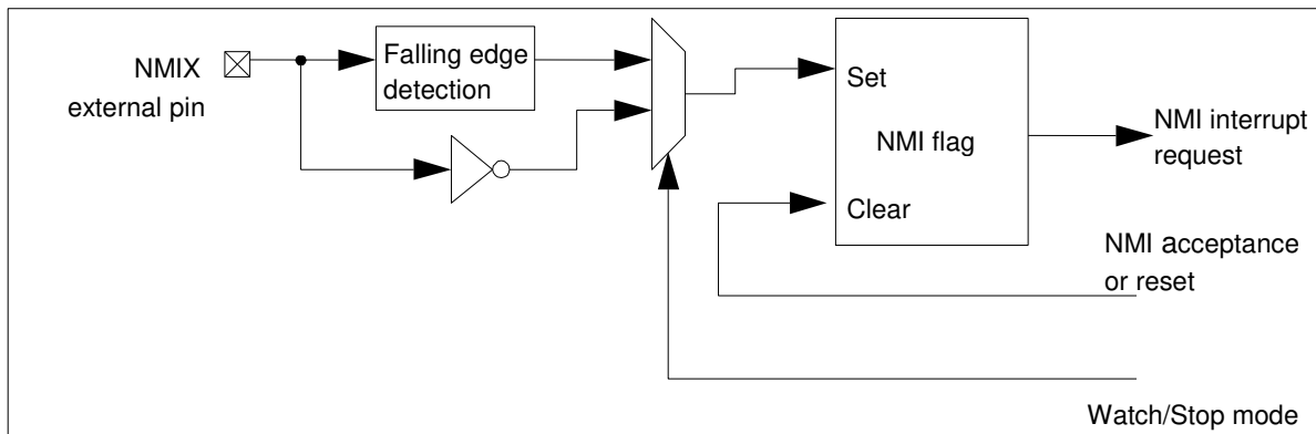
Figure 3-1 Block Diagram
