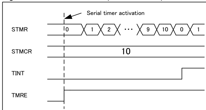
Figure 5-10 Start by Using Serial Timer Enable Bit (STMCR="10")
