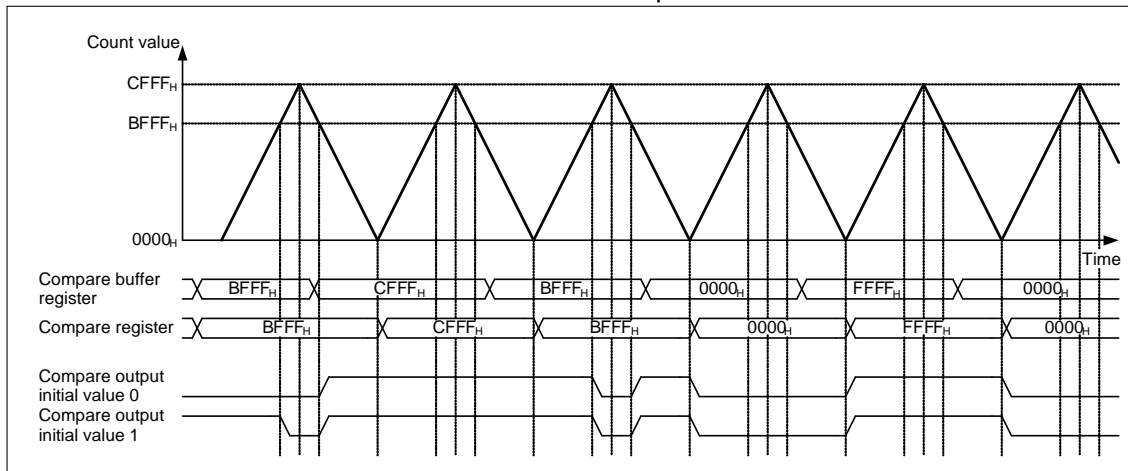
Figure 5-18 Case #6 Where the Free-run Timer Is in Up/Down Count Mode
