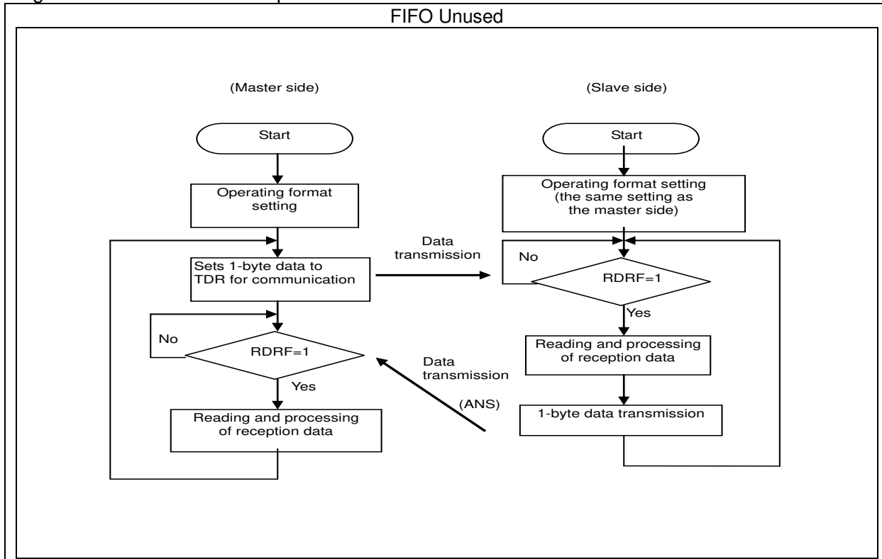
Figure 6-30 Flowchart Example
