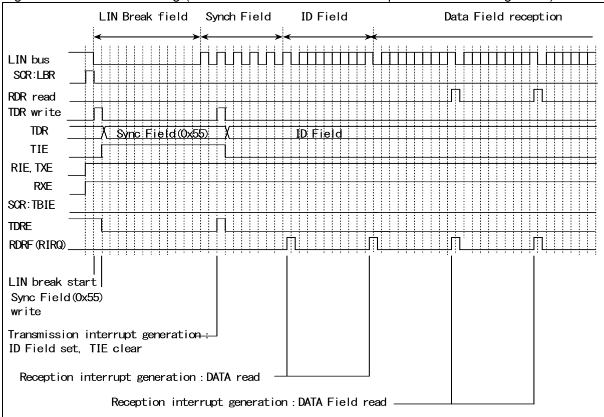
Figure 7-30 LIN Bus Timing (at the Time of Data Field Reception without Using FIFO)
