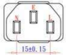
插頭端面圖 (Dimensions of Plug Face)
