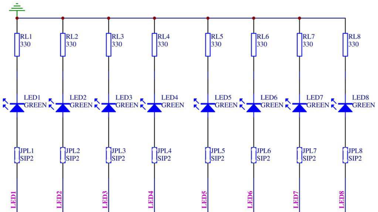
Figure 2-3. Circuit Diagram of the LEDs and Jumpers
