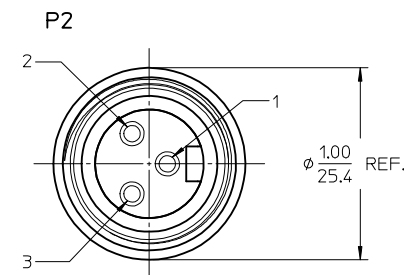
FACE VIEW MALE SCALE: 2X
