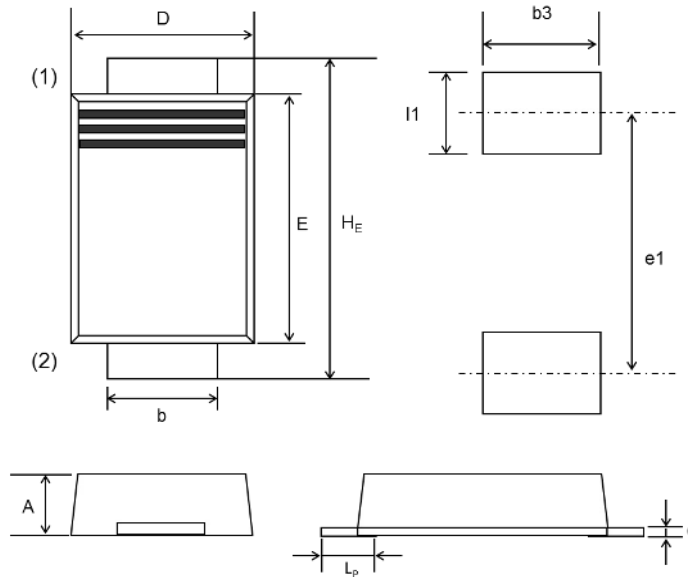
SOD-128, (PVD™)
