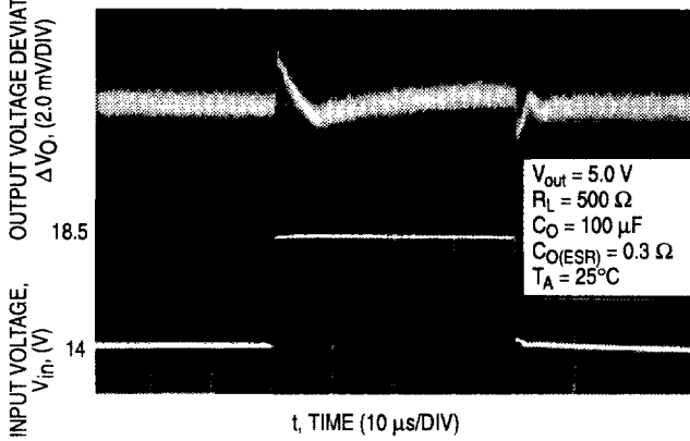
Figure 13. Line Regulation
