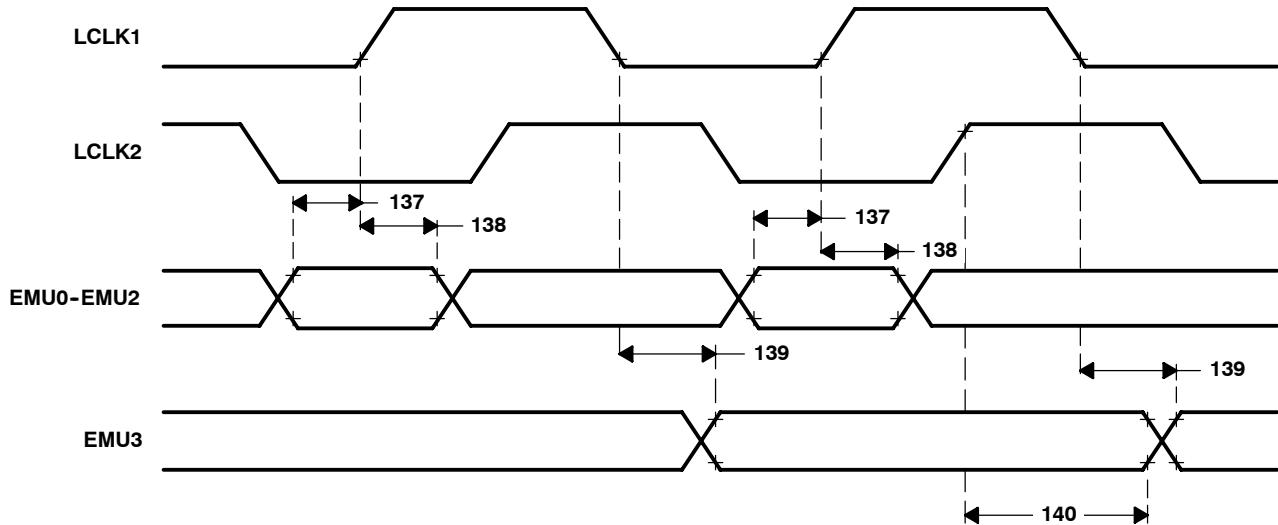
Figure 58. Emulator-Interface Timing
