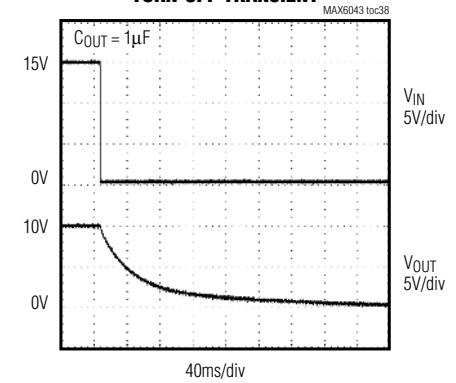
TURN-OFF TRANSIENT
