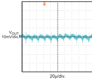
Output Ripple
