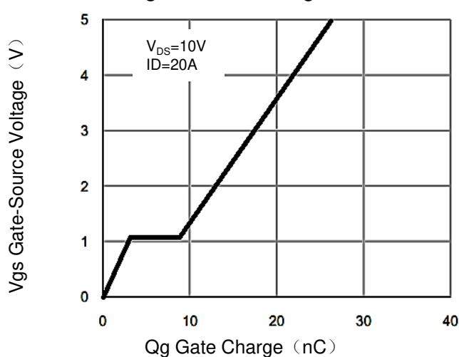
Figure 3. Gate Charge
