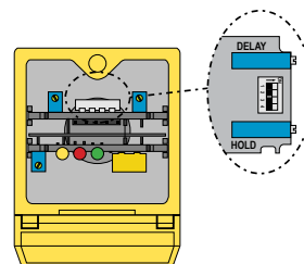
Figure 1. DIP switches for programming Delay logic
