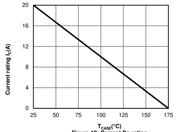
Figure 12: Current De-rating
