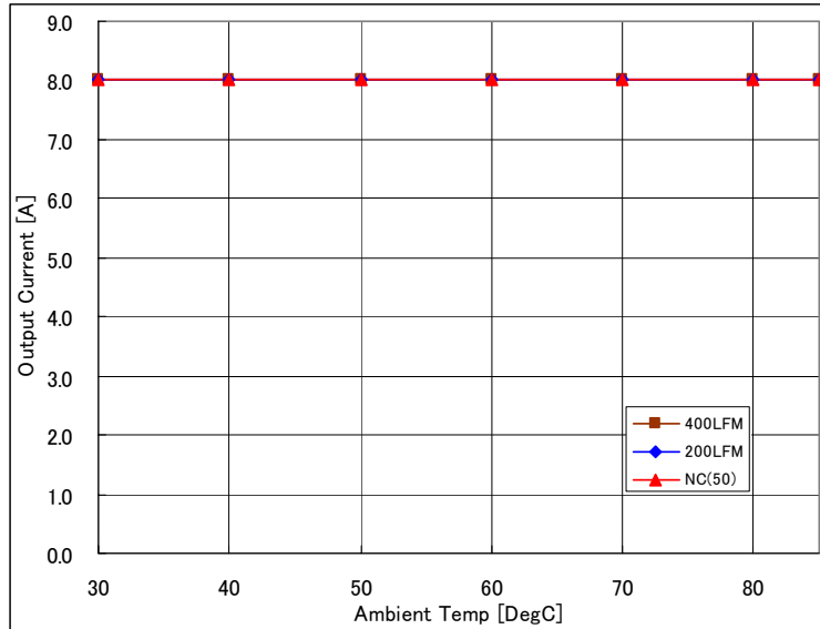
Fig 3.3V-1: Available load current vs. ambient temperature and airflow rates for Vout=3.3V with Vin=12V. Maximum component temperature \leq 120^{\circ}\text{C} .
