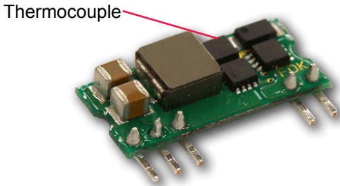
Fig. C: Location of the thermocouple for thermal testing
