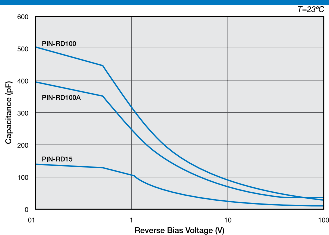
Typical Capacitance vs. Reverse Bias Voltage
