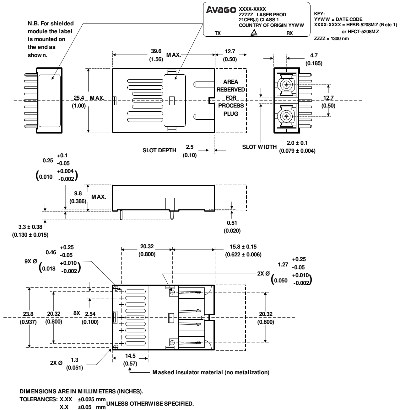
Figure 7a. Package Outline Drawing for HFBR/HFCT-5208xxxZ
