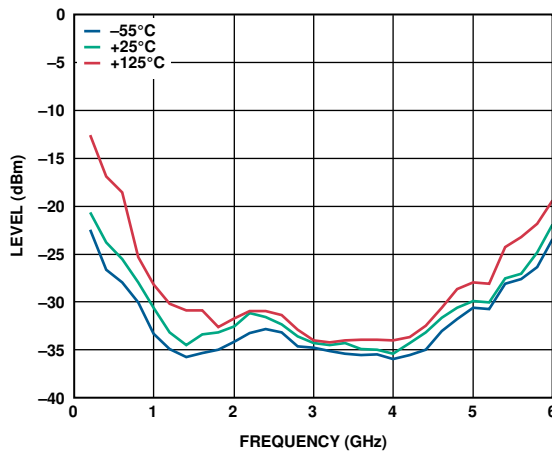
Figure 6. Input Sensitivity
