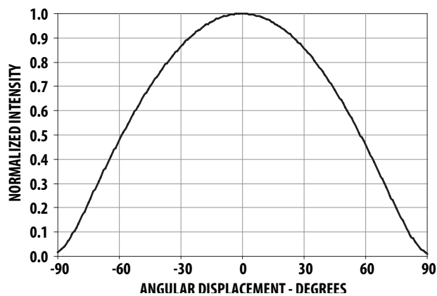
Figure 11. Radiation Pattern
