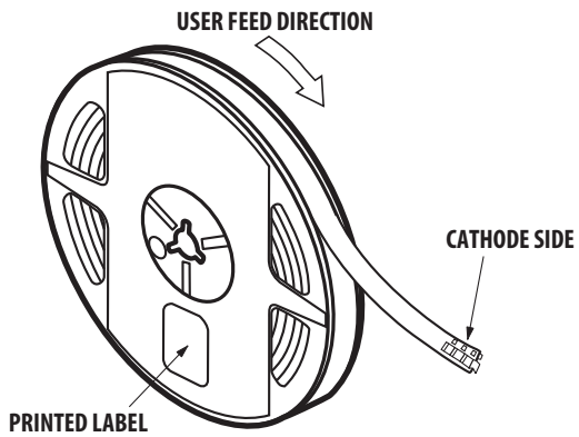
Figure 17. Reeling Orientation
