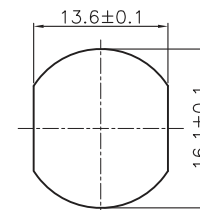
M16 Recommended Panel CUT-Out Thickness 4.0 Max.
