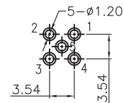
2~5P Recommended PCB Layout TOL:±0.05mm
