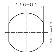
PG9 Recommended Panel CUT-Out Thickness 4.0 Max.
