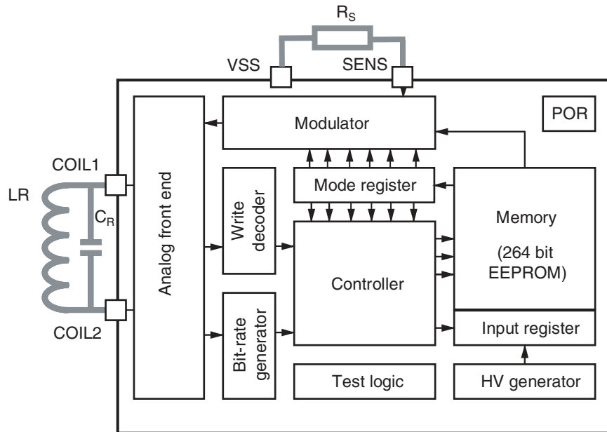
Figure 4-1. Block Diagram
