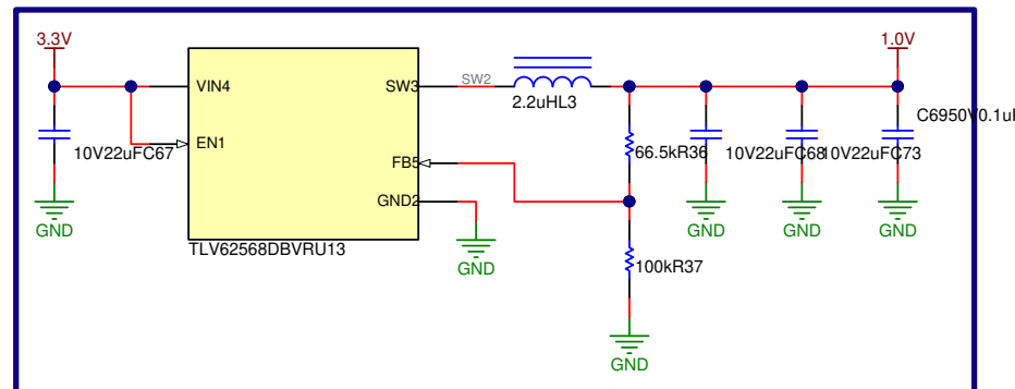
Figure 11. EVM Power
