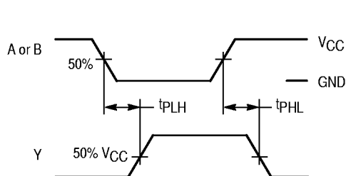
Figure 1. Switching Waveforms
