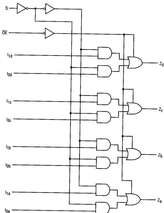
LOGIC DIAGRAM
