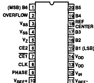
CA3306 (SOIC) TOP VIEW
