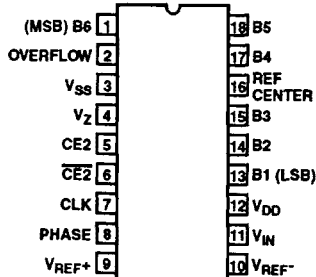
CA3306 (PDIP, CDIP) TOP VIEW
