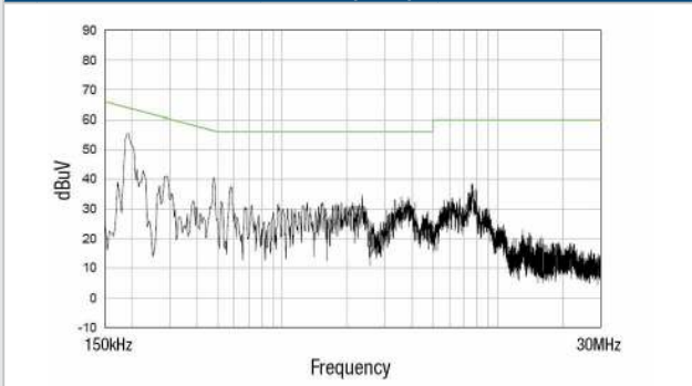
BAC1S12SC (110V) - Live
