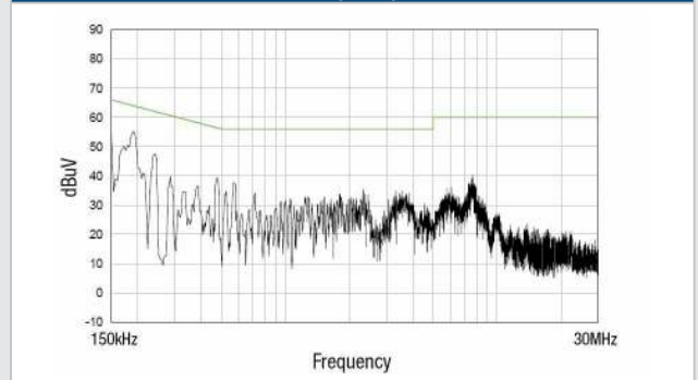
BAC1S12SC (110V) - Neutral
