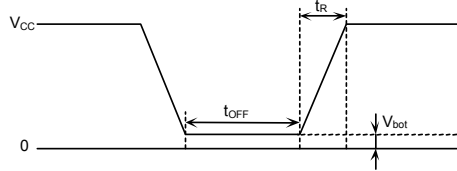
Figure 48. Rise Waveform Diagram
