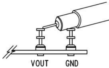
Figure 7. Measure Output Ripple
