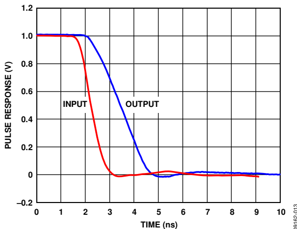
Figure 13. Negative Pulse Response, 1 V to 0 V
