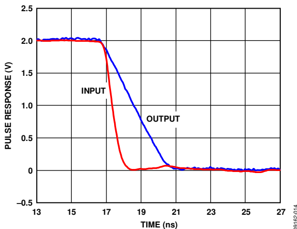
Figure 14. Negative Pulse Response, 2 V to 0 V
