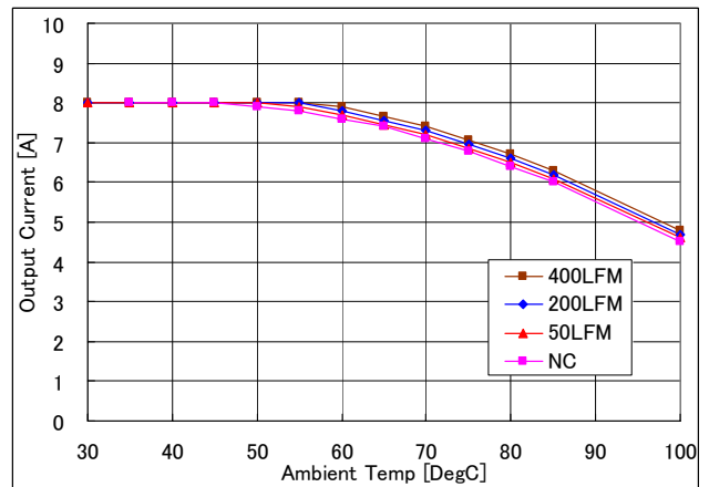
Fig.2: Output current vs. ambient temperature and air velocity at 5.0V in , 2.5V out
