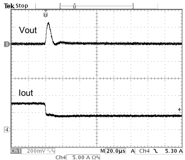
Fig.22: Output voltage response to step load change at 5A/us from 100% to 50% (5.0Vin, 0.8Vout)
