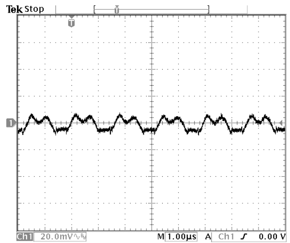
Fig.20: Output ripple and noise at 5.0Vin, 0.8V/8Aout
