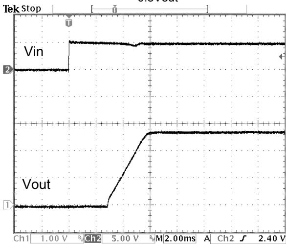
Fig.15: Turn on delay time at 5.0Vin, 2.75V/8A out
