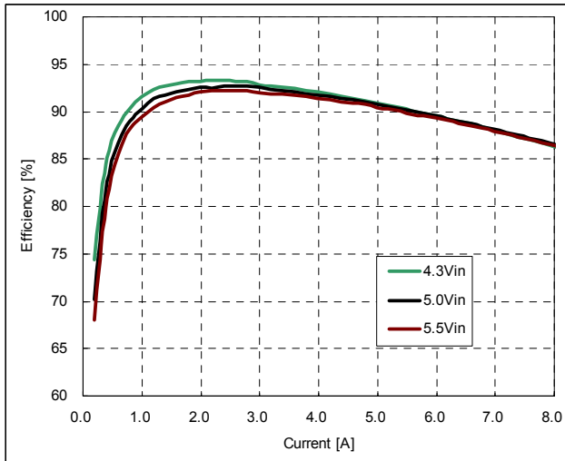
Fig.8: Efficiency vs. load current and input voltage for 2.75Vout
