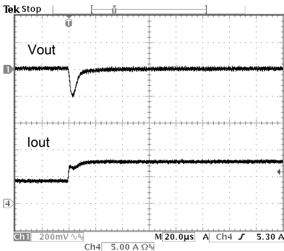
Fig.21: Output voltage response to step load change at 5A/us from 50% to 100% (5.0Vin, 0.8Vout)
