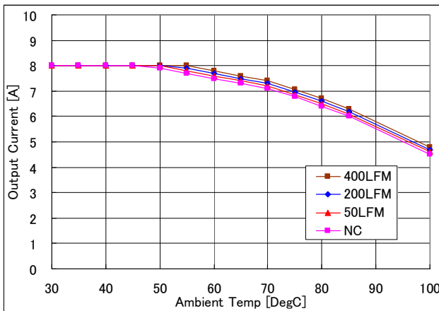
Fig.1: Output current vs. ambient temperature and air velocity at 5.0V in , 2.75V out
