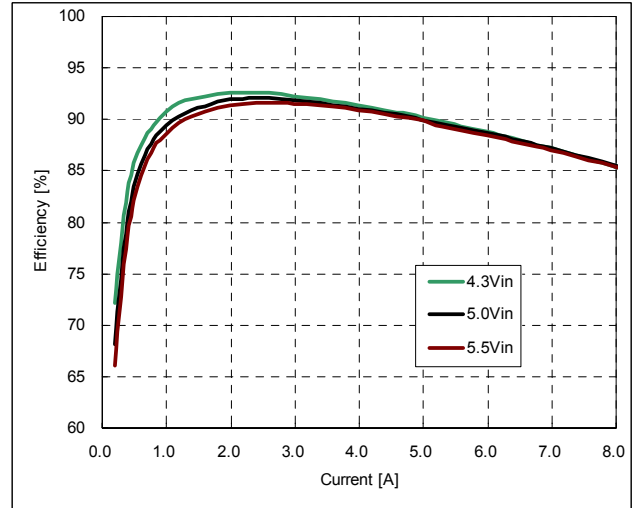
Fig.9: Efficiency vs. load current and input voltage for 2.5Vout
