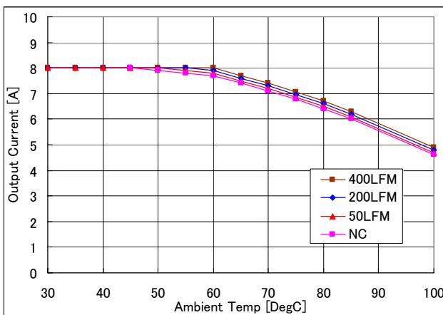
Fig.3: Output current vs. ambient temperature and air velocity at 5.0V in , 1.8V out
