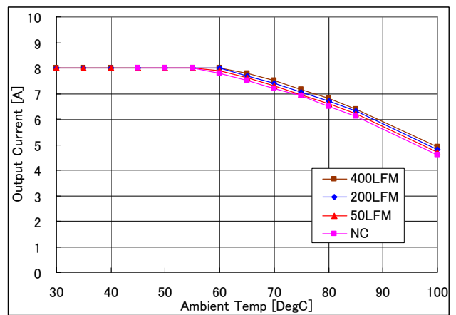
Fig.4: Output current vs. ambient temperature and air velocity at 5.0V in , 1.5V out
