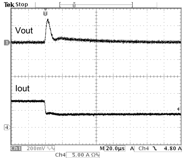
Fig.18: Output voltage response to step load change at 5A/us from 100% to 50% (5.0Vin, 2.75Vout)
