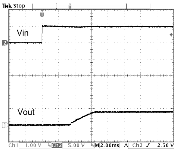
Fig.19: Turn on delay time at 5.0Vin, 0.8V/8A out
