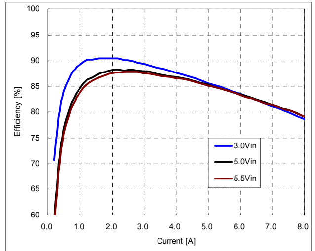
Fig.11: Efficiency vs. load current and input voltage for 1.5Vout
