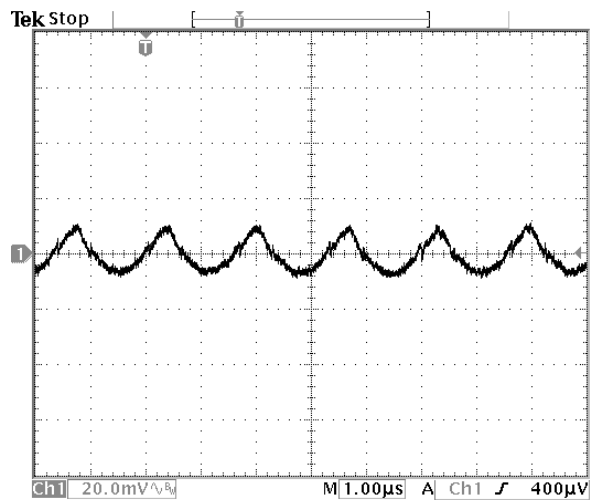
Fig.16: Output ripple and noise at 5.0Vin, 2.75V/8Aout
