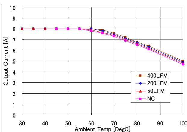
Fig.5: Output current vs. ambient temperature and air velocity at 5.0V in , 1.2V out
