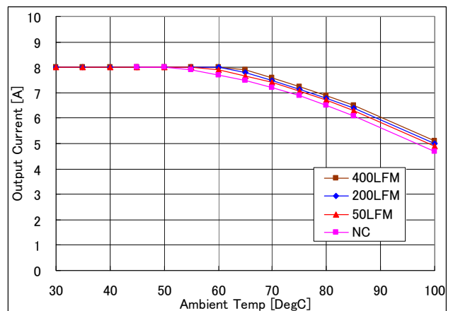
Fig.6: Output current vs. ambient temperature and air velocity at 5.0V in , 1.0V out
