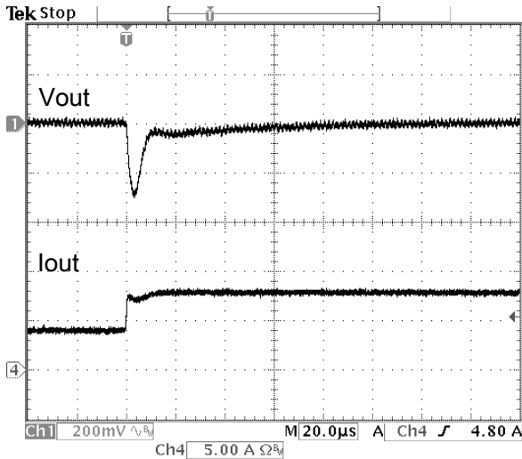
Fig.17: Output voltage response to step load change at 5A/us from 50% to 100% (5.0Vin, 2.75Vout)
