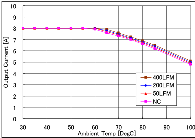
Fig.7: Output current vs. ambient temperature and air velocity at 5.0Vin, 0.8V out
