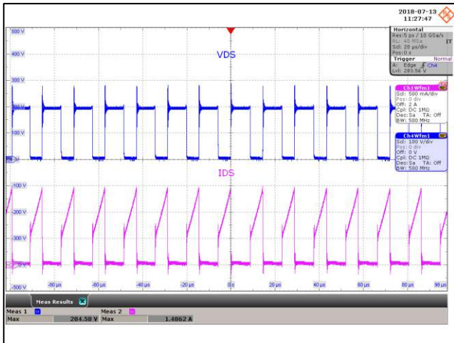
Figure 69 – Drain Voltage and Current Waveforms. 85 VAC, 8.0 V, 5 A Load (284 V MAX ). Upper: V DRAIN , 100 V / div., 20 µs / div. Lower: I DRAIN , 500 mA / div.
