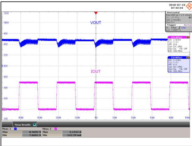
Figure 59 – Transient Response. 85 VAC, 8.0 V, 0 - 5 A Load Step. V_{MIN} : 7.66 V, V_{MAX} : 8.56 V. Upper: V_{OUT} , 1 V / div., 1 ms / div. Lower: I_{LOAD} , 2 A / div.
