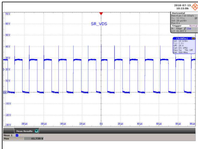
Figure 83 – SR FET Voltage Waveforms. 85 VAC, 15.0 V, 2.66 A Load (41.73 V_{MAX} ). SR_V DRAIN , 10 V / div., 20 \mu s / div.
