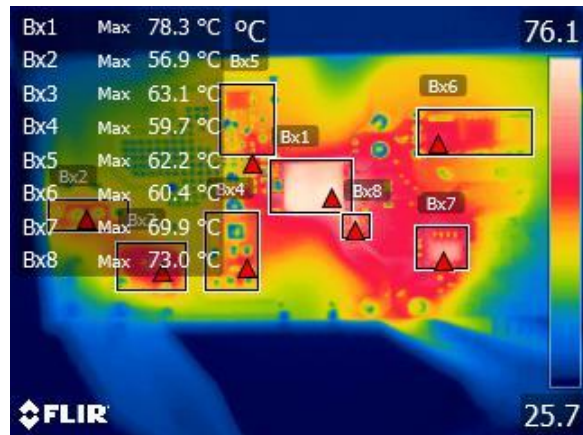
Figure 40 – Bottom Components, Ambient = 27 °C. Bx1: InnoSwitch3-Pro = 78.3 °C. Bx2: Bridge Diodes, PCB = 56.9 °C. Bx3: Thermistor, PCB = 63.1 °C. Bx4: Primary Snubber = 59.7 °C. Bx5: Auxiliary Circuit = 62.2 °C. Bx6: SR FET = 60.4 °C. Bx7: Pass FET = 69.9 °C. Bx8: Current Sense Resistor = 73.0 °C.
