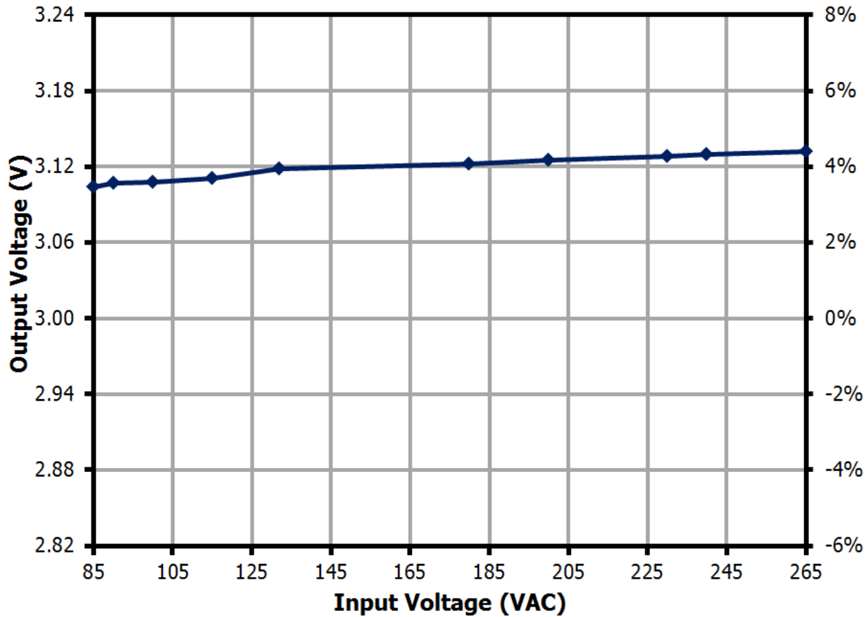
Figure 19 – 3 V Output Regulation vs. Input Line Voltage.
