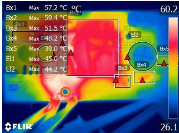
Figure 41 – Top Components, Ambient = 27 °C. Bx1: SR FET, PCB = 57.2 °C. Bx2: Transformer = 59.4 °C. Bx3: Primary Snubber = 51.5 °C. Bx4: Thermistor = 48.2 °C. Bx5: Bridge Diodes = 39.0 °C. E11: Output Capacitor = 45.0 °C. E12: Input Capacitor = 44.2 °C.
