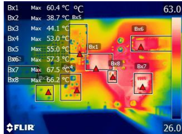
Figure 42 – Bottom Components, Ambient = 27 °C. Bx1: InnoSwitch3-Pro = 60.4 °C. Bx2: Bridge Diodes, PCB = 38.7 °C. Bx3: Thermistor, PCB = 44.1 °C. Bx4: Primary Snubber = 53.0 °C. Bx5: Auxiliary Circuit = 55.0 °C. Bx6: SR FET = 57.3 °C. Bx7: Pass FET = 67.5 °C. Bx8: Current Sense Resistor = 66.2 °C.
