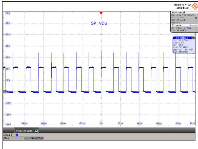
Figure 81 – SR FET Voltage Waveforms. 85 VAC, 8.0 V, 5 A Load (34.62 V_{MAX} ). SR_V DRAIN , 10 V / div., 20 \mu s / div.
