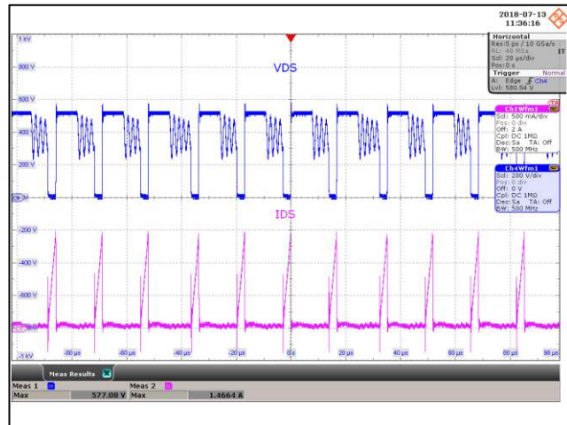
Figure 72 – Drain Voltage and Current Waveforms. 265 VAC, 15.0 V, 2.66 A Load (577 V MAX ). Upper: V DRAIN , 200 V / div., 20 µs / div. Lower: I DRAIN , 500 mA / div.
