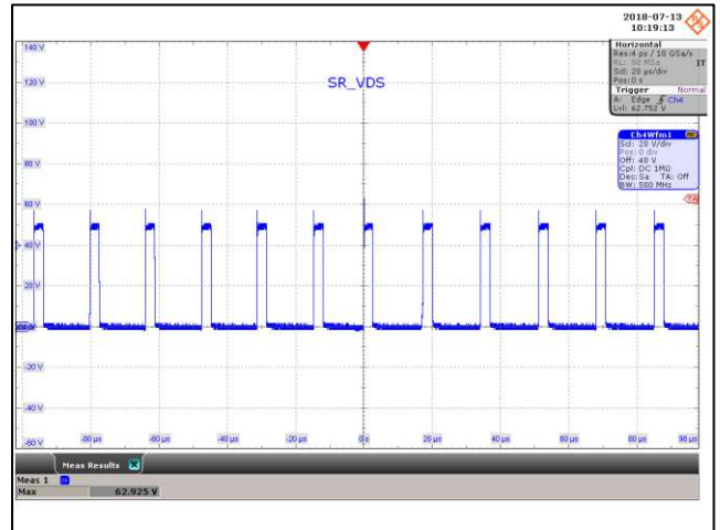
Figure 82 – SR FET Voltage Waveforms. 265 VAC, 8.0 V, 5 A Load (62.92 V_{MAX} ). SR_V DRAIN , 20 V / div., 20 \mu s / div.
