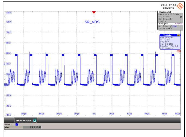
Figure 84 – SR FET Voltage Waveforms. 265 VAC, 15.0 V, 2.66 A Load (63.71 V_{MAX} ). SR_V DRAIN , 20 V / div., 20 \mu s / div.
