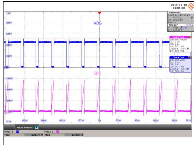
Figure 70 – Drain Voltage and Current Waveforms. 265 VAC, 8.0 V, 5 A Load (521 V MAX ). Upper: V DRAIN , 200 V / div., 20 µs / div. Lower: I DRAIN , 500 mA / div.
