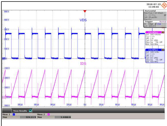
Figure 71 – Drain Voltage and Current Waveforms. 85 VAC, 15.0 V, 2.66 A Load (324 V MAX ). Upper: V DRAIN , 100 V / div., 20 µs / div. Lower: I DRAIN , 500 mA / div.
