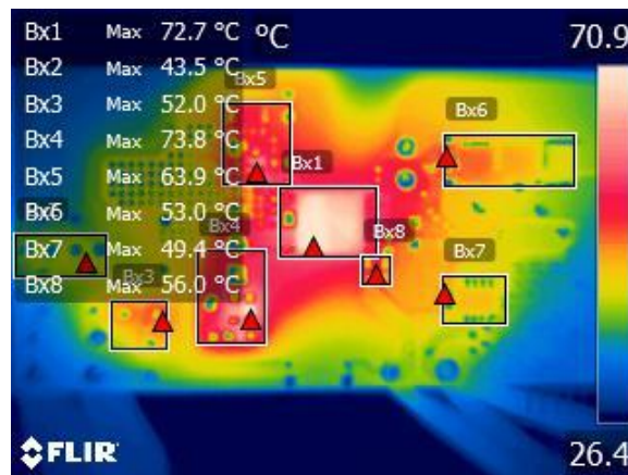
Figure 50 – Bottom Components, Ambient = 27 °C. Bx1: InnoSwitch3-Pro = 72.7 °C. Bx2: Bridge Diodes, PCB = 43.5 °C. Bx3: Thermistor, PCB = 52.0 °C. Bx4: Primary Snubber = 73.8 °C. Bx5: Auxiliary Circuit = 63.9 °C. Bx6: SR FET = 53.0 °C. Bx7: Pass FET = 49.4 °C. Bx8: Current Sense Resistor = 56.0 °C.
