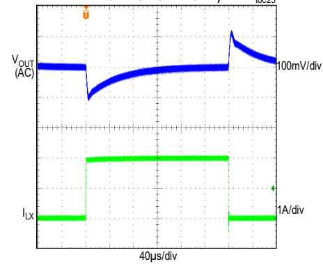
3.3V OUTPUT, PWM MODE, FIGURE 4 CIRCUIT (LOAD CURRENT STEPPED FROM NO LOAD TO 2A)
