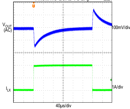
5V OUTPUT, PWM MODE, FIGURE 3 CIRCUIT (LOAD CURRENT STEPPED FROM NO LOAD TO 2A)
