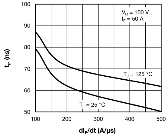
Fig. 8 - Typical Reverse Recovery Time vs di/dt (Per Diode)
