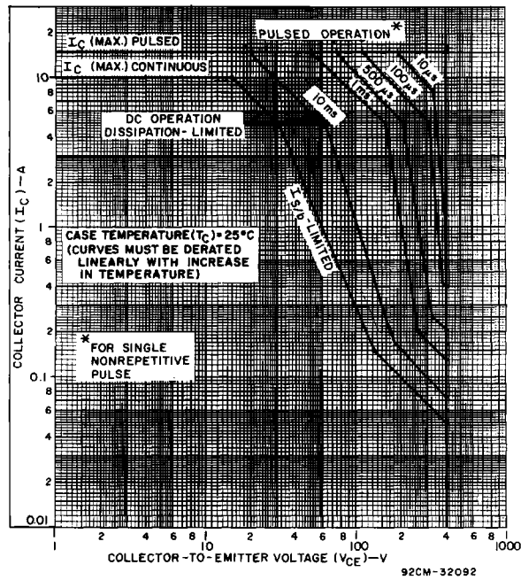
Fig. 3 — Maximum safe-operating areas ( T_c = 25^\circ\text{C} ).
