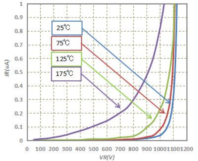
Fig.2-Typical Reverse Characteristics
