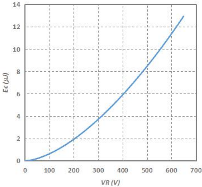
Fig.5-Capacitance Stored Energy
