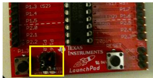
Figure 10. LaunchPad J5 Header Connections
