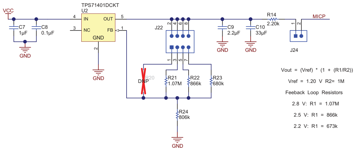
Figure 6. On-Board MICBIAS Output
