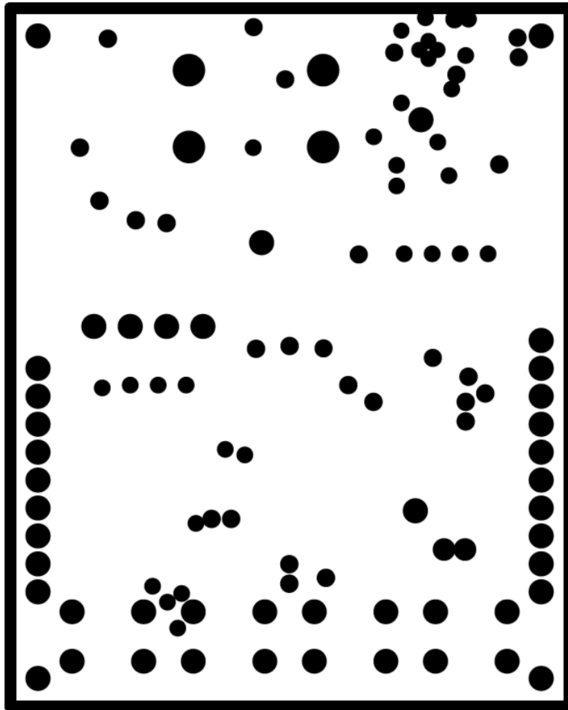
Figure 24. Power Plane (Negative Image)
