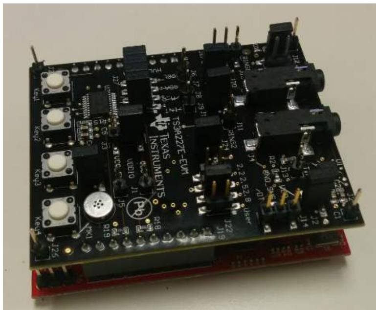
Figure 15. LaunchPad to EVM Connection
