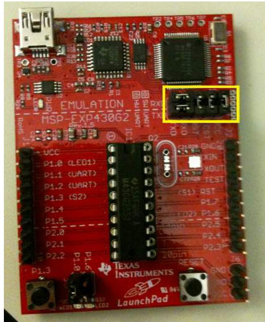
Figure 9. LaunchPad Header Connections
