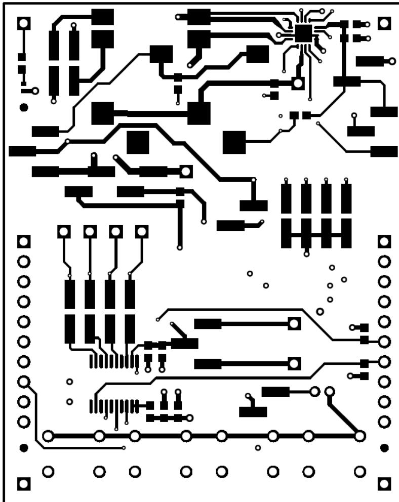
Figure 22. Top Copper
