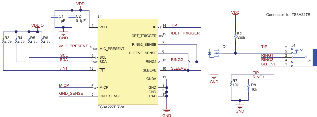
Figure 2. Connector to TS3A227E
