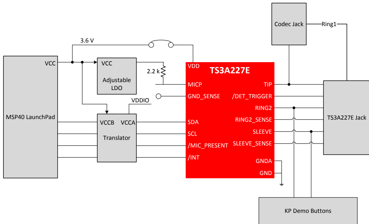
Figure 1. TS3A227E-EVM Block Diagram
