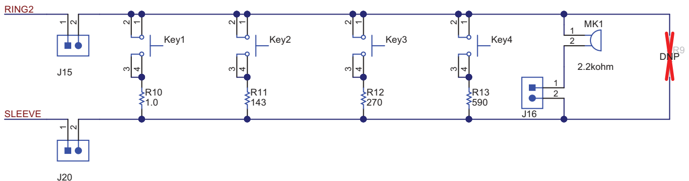
Figure 7. Key Press Schematic
