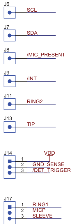
Figure 4. Breakout Test Point Headers
