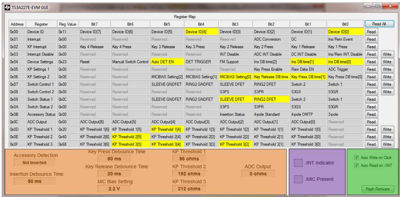
Figure 18. TS3A227E-EVM GUI Details
