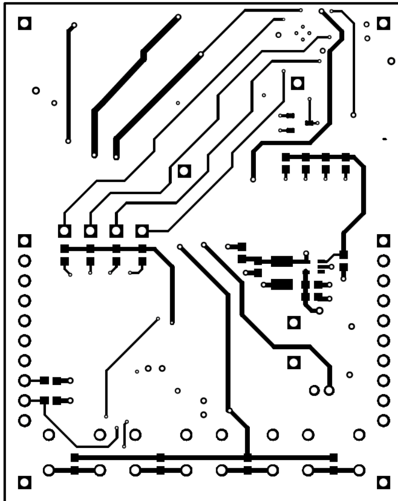
Figure 25. Bottom Copper
