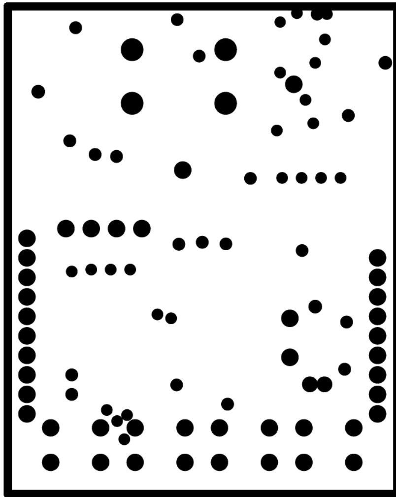
Figure 23. Ground Plane (Negative Image)
