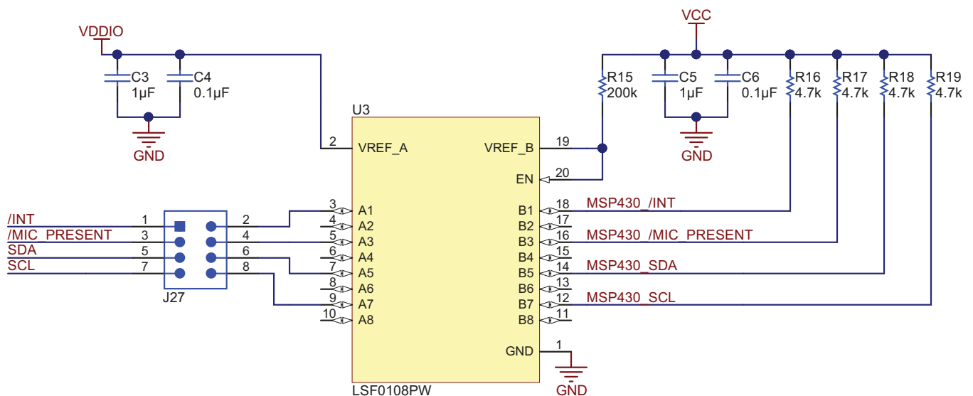
Figure 5. Translator
