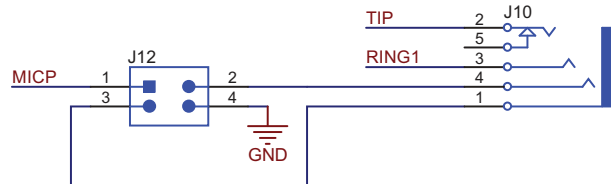
Figure 8. External CODEC Interface
