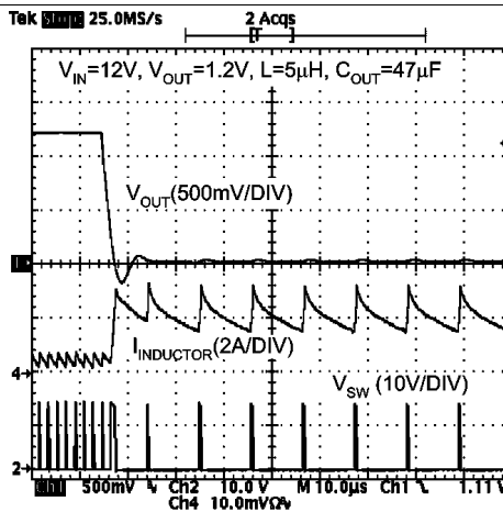
Figure 22. Short-Circuit Triggering
