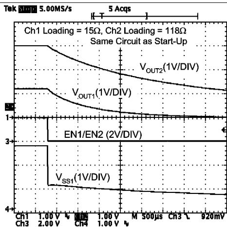
Figure 19. Shutdown
