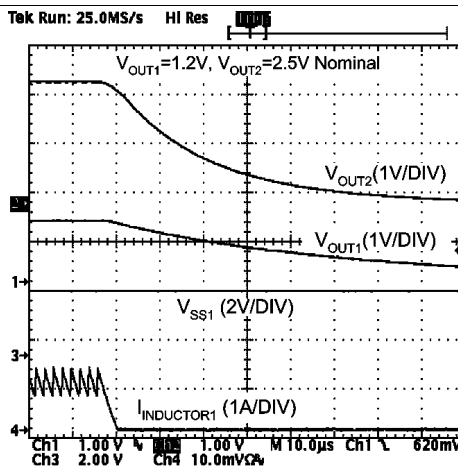
Figure 20. Thermal Shutdown
