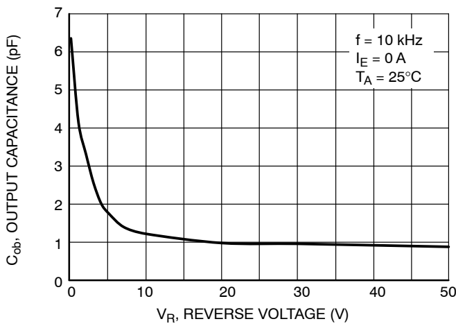
Figure 19. Output Capacitance
