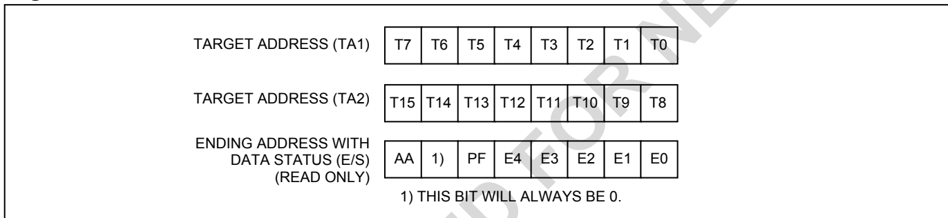
Figure 6. ADDRESS REGISTER
