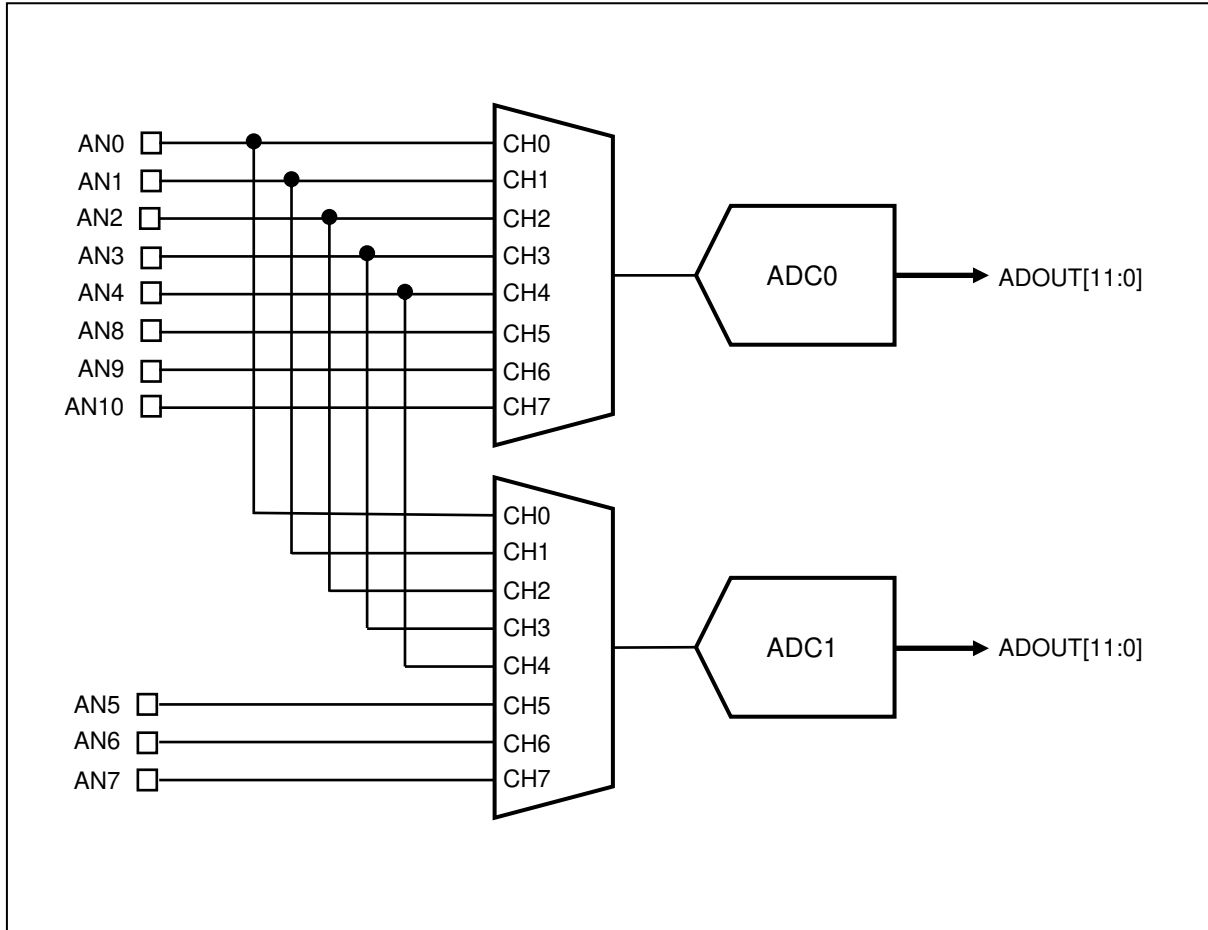
Figure 16.2 Analog Channel Block Diagram
