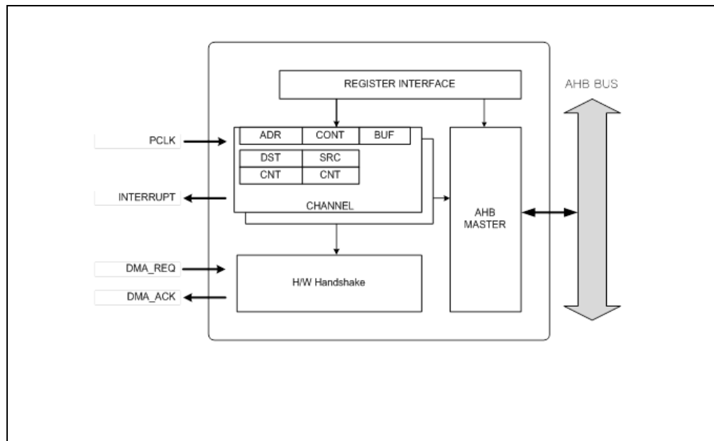
Figure 9.1 Block Diagram
