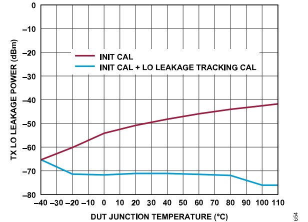
Figure 104. Transmitter LO Leakage Power vs. DUT Junction Temperature (Low to High), Baseband Frequency = 4 MHz, Backoff = 0.5 dBFS, Attenuation Code = 0
