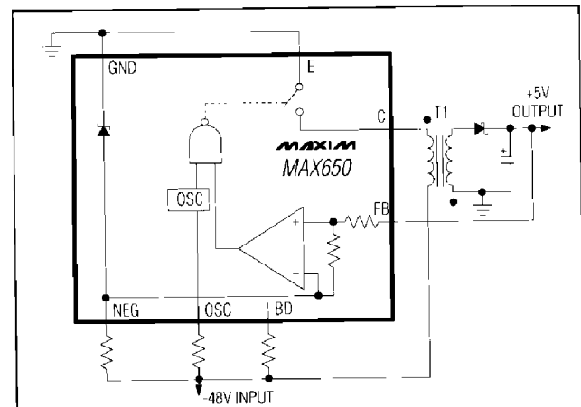
Figure 3. Typical Circuit
