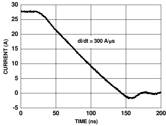
Figure 14. FDMS0343S SyncFET body diode reverse recovery characteristic
