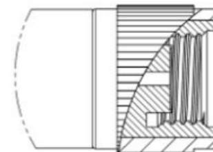
CONNECTOR:RP-SMA(M)
