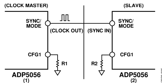
Figure 35. Two ADP5056 Devices Configured for Synchronization Mode
