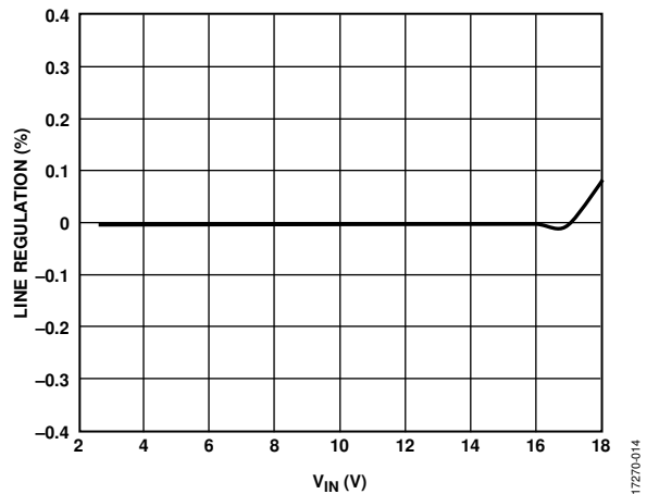
Figure 14. Channel 3 Line Regulation, V_{OUT} = 1.2\text{ V} , I_{OUT} = 3\text{ A} , f_{SW} = 600\text{ kHz} , FPWM Mode
