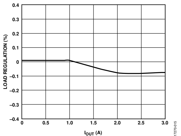
Figure 15. Channel 3 Load Regulation, V_{IN} = 12\text{ V} , V_{OUT} = 1.2\text{ V} , f_{SW} = 600\text{ kHz} , FPWM Mode
