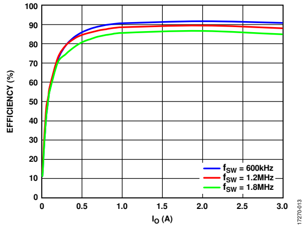
Figure 13. Channel 3 Efficiency Curve, V_{IN} = 12\text{ V} , V_{OUT} = 3.3\text{ V} , FPWM Mode (600 kHz, 1.2 MHz, 1.8 MHz)
