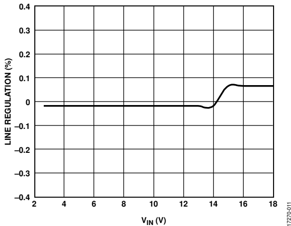
Figure 11. Channel 1/Channel 2 Line Regulation, V_{OUT} = 1.2\text{ V} , I_{OUT} = 7\text{ A} , f_{SW} = 600\text{ kHz} , FPWM Mode
