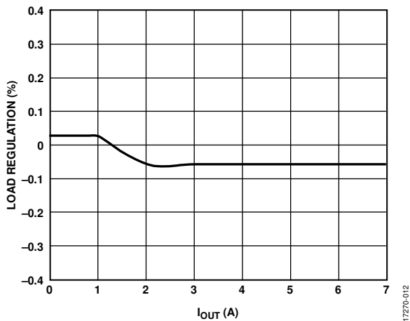
Figure 12. Channel 1/Channel 2 Load Regulation, V_{IN} = 12\text{ V} , V_{OUT} = 1.2\text{ V} , f_{SW} = 600\text{ kHz} , FPWM Mode
