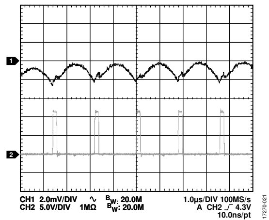
Figure 21. Channel 1/Channel 2 Steady State Waveform, V IN = 12 V, V OUT = 1.2 V, I OUT = 7 A, f SW = 600 kHz, L = 1 μH, C OUT = 47 μF × 6, FPWM Mode, Channel 1 = V OUT , Channel 2 = Switching Point (SW)
