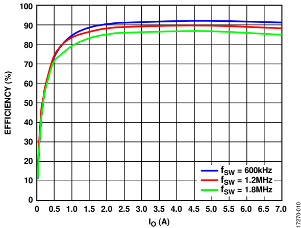
Figure 10. Channel 1/Channel 2 Efficiency Curve, V_{IN} = 12\text{ V} , Output Voltage ( V_{OUT} ) = 3.3 V, FPWM Mode (600 kHz, 1.2 MHz, 1.8 MHz)
