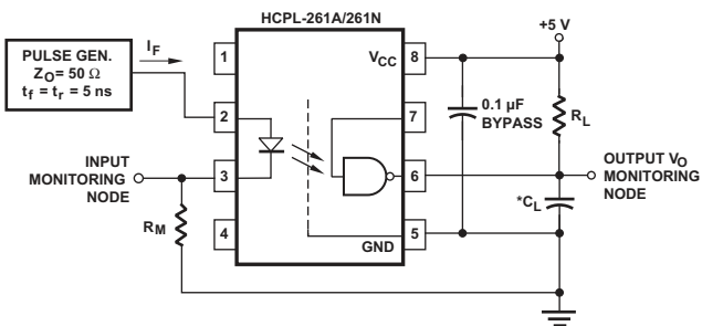
Figure 10: Test Circuit for t pHL and t pLH
