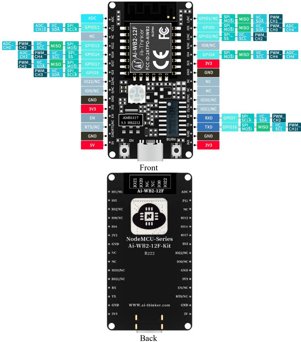
Figure 6 pin diagram
