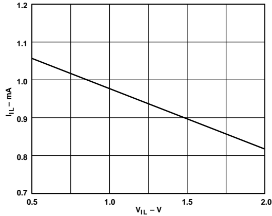
Figure 23. Input Characteristics of Pin 6 When Pulled Low Pin 7 (SYNC)
