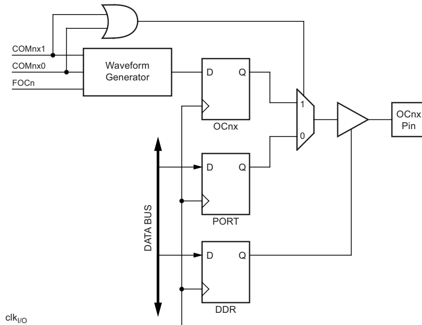
Figure 4-29. Compare Match Output Unit, Schematic
