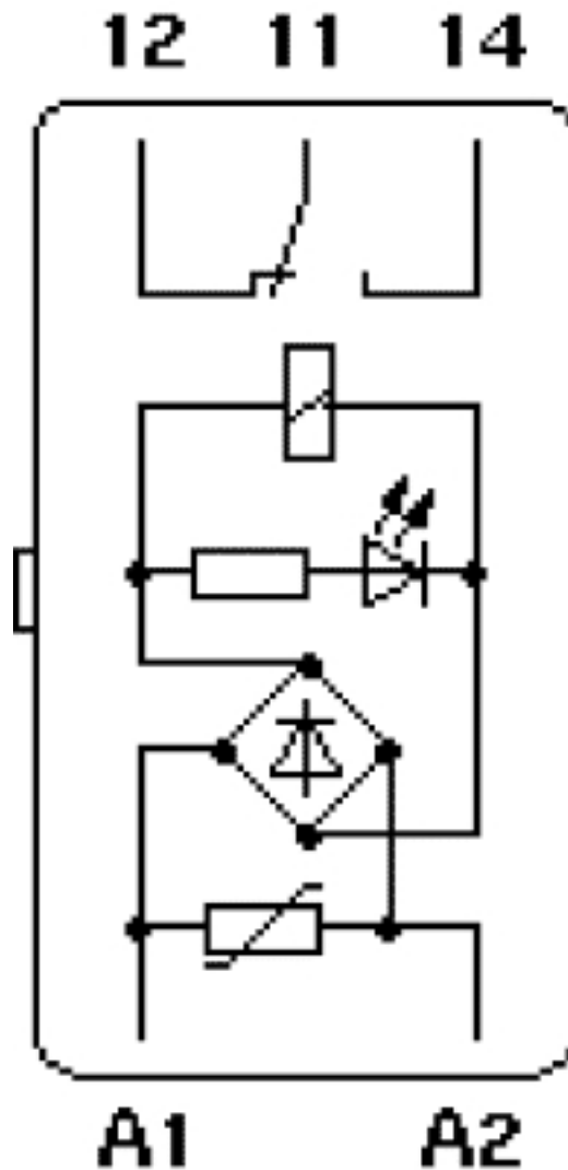
Circuit diagram
