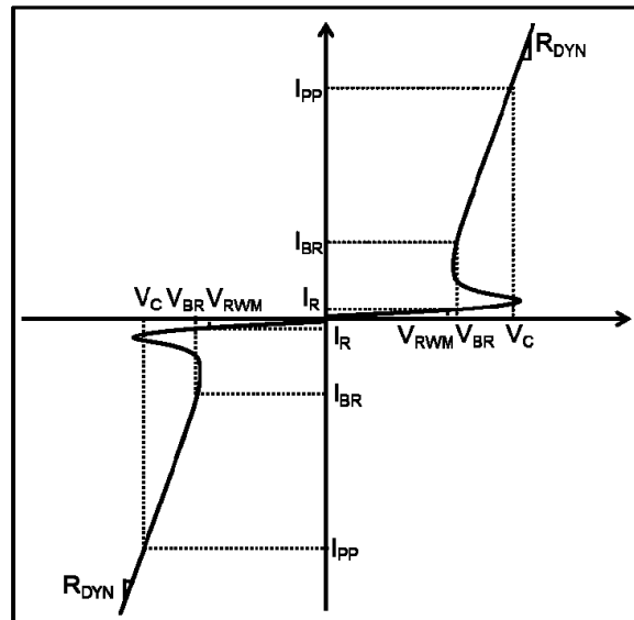
Fig. 7.1 Definitions of Electrical Characteristics
