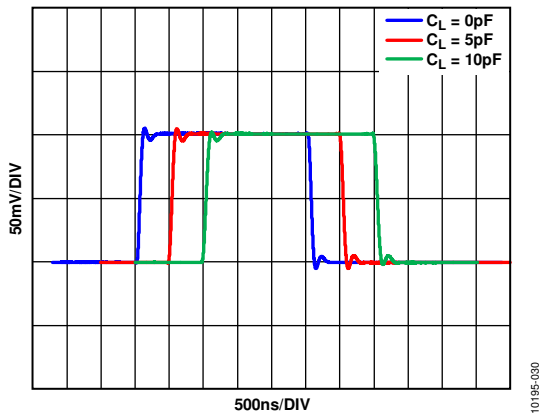
Figure 30. Small Signal Step Response for Various Capacitive Loads, V_S = \pm 5\text{ V}
