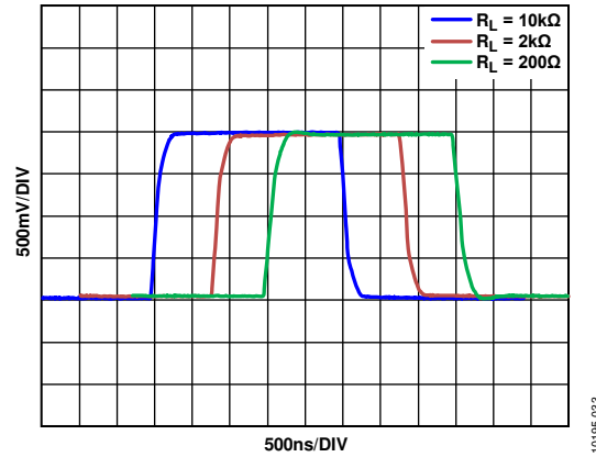
Figure 32. Large Signal Step Response for Various Resistive Loads, V_S = \pm 5\text{ V}
