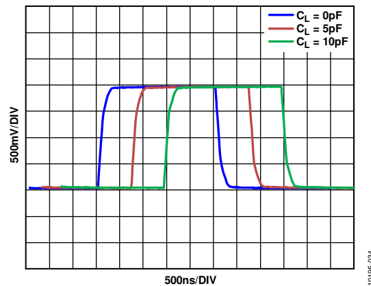
Figure 33. Large Signal Step Response for Various Capacitive Loads, V_S = \pm 5\text{ V}
