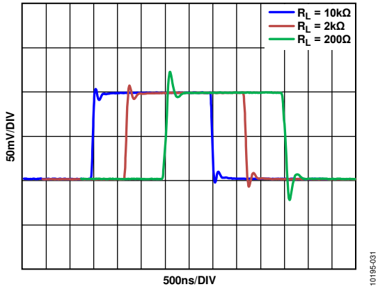
Figure 29. Small Signal Step Response for Various Resistive Loads, V_S = \pm 5\text{ V}
